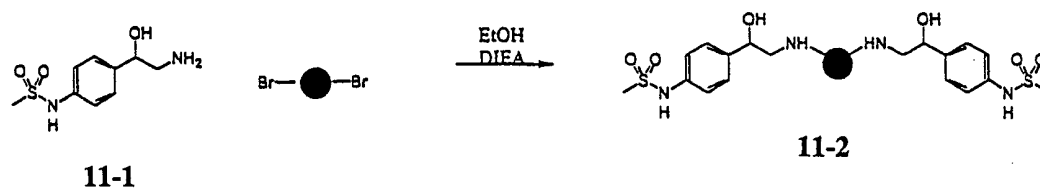
Figure 11. Reaction Schemes for Bivalent Sotalol Compounds
