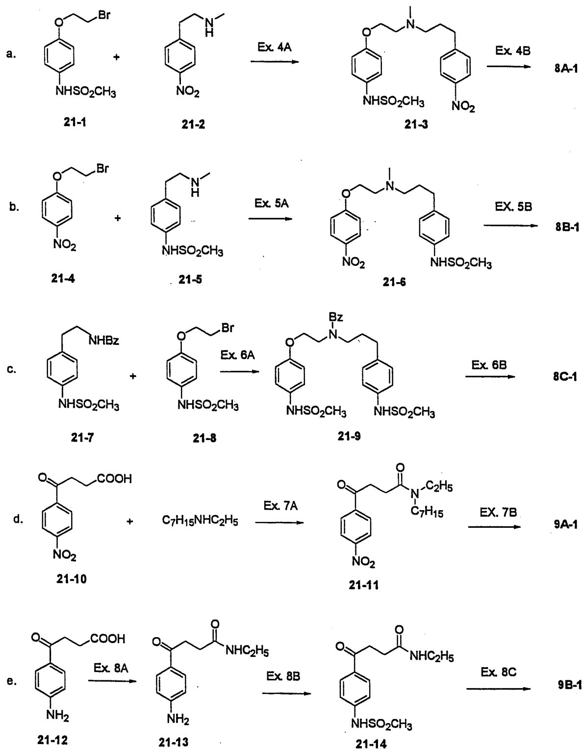
Figure 21. Preparation of Intermediates
