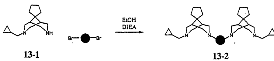
Figure 13. Reaction Schemes for Bivalent Tedasimil Compounds
