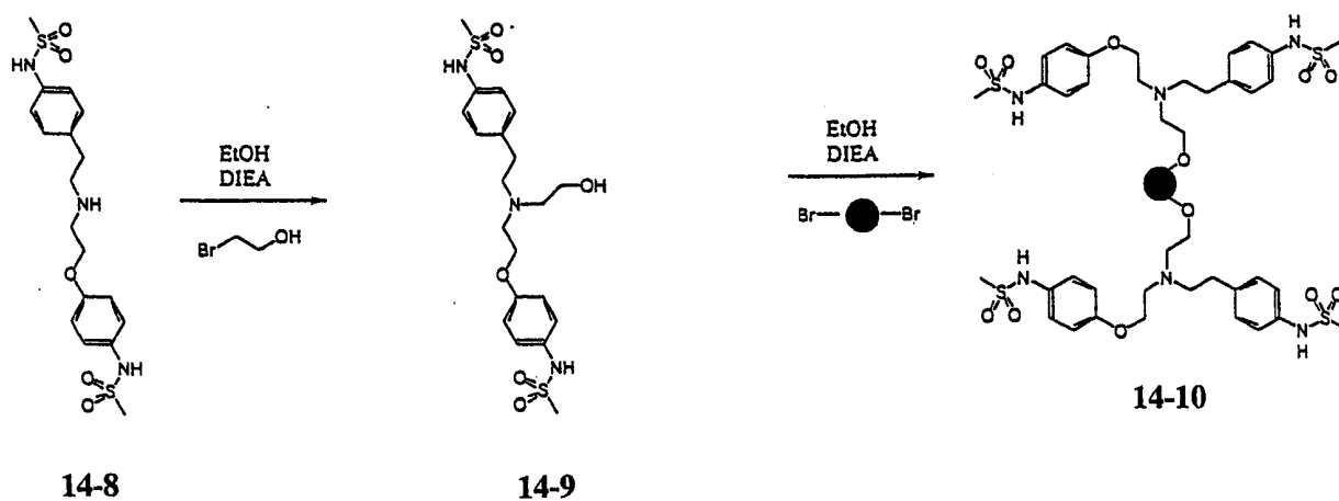
Figure 14. Introduction of Spacer to Facilitate Multivalomer Formation
