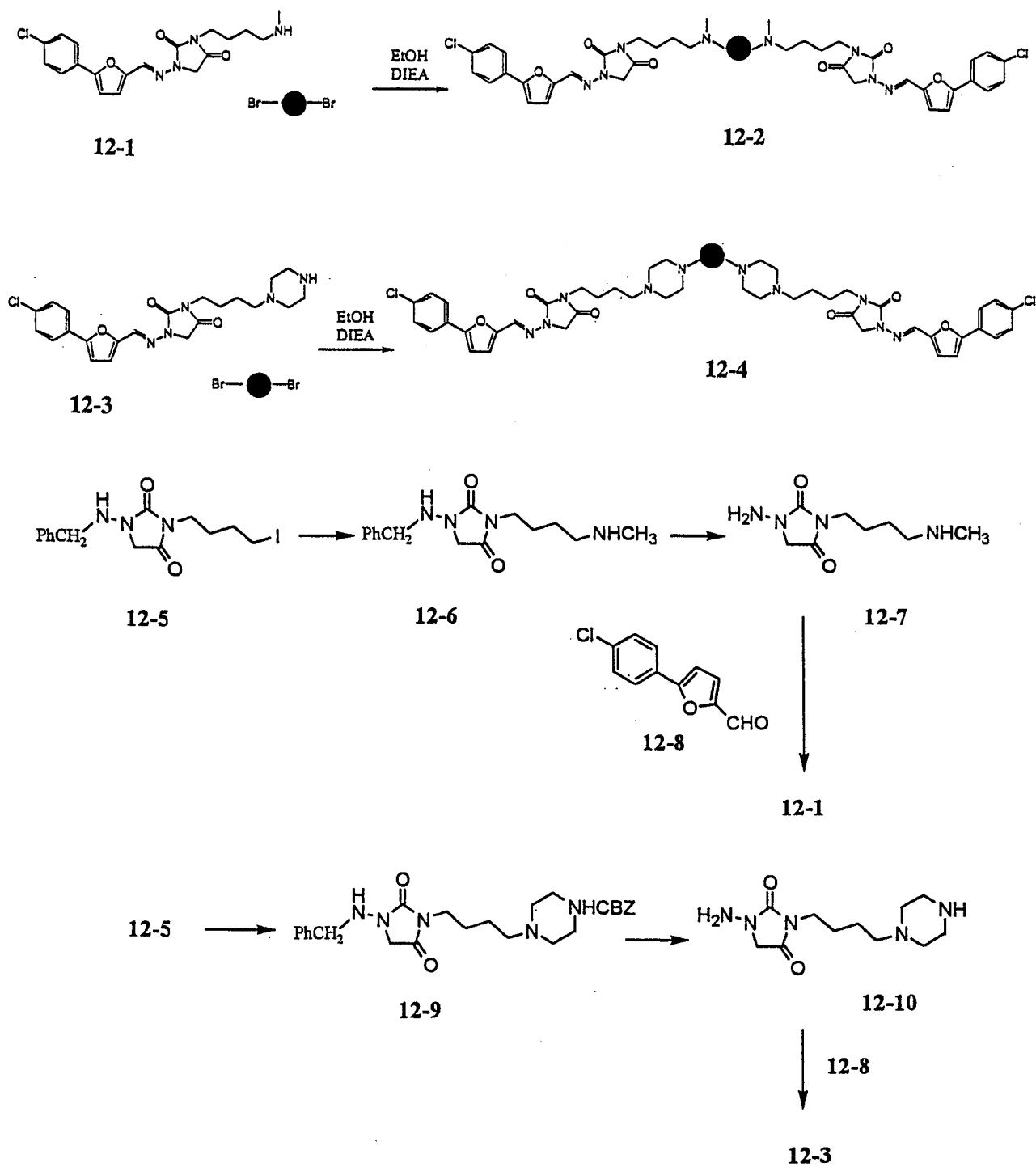
Figure 12. Reaction Schemes for Bivalent Azimilide Compounds
