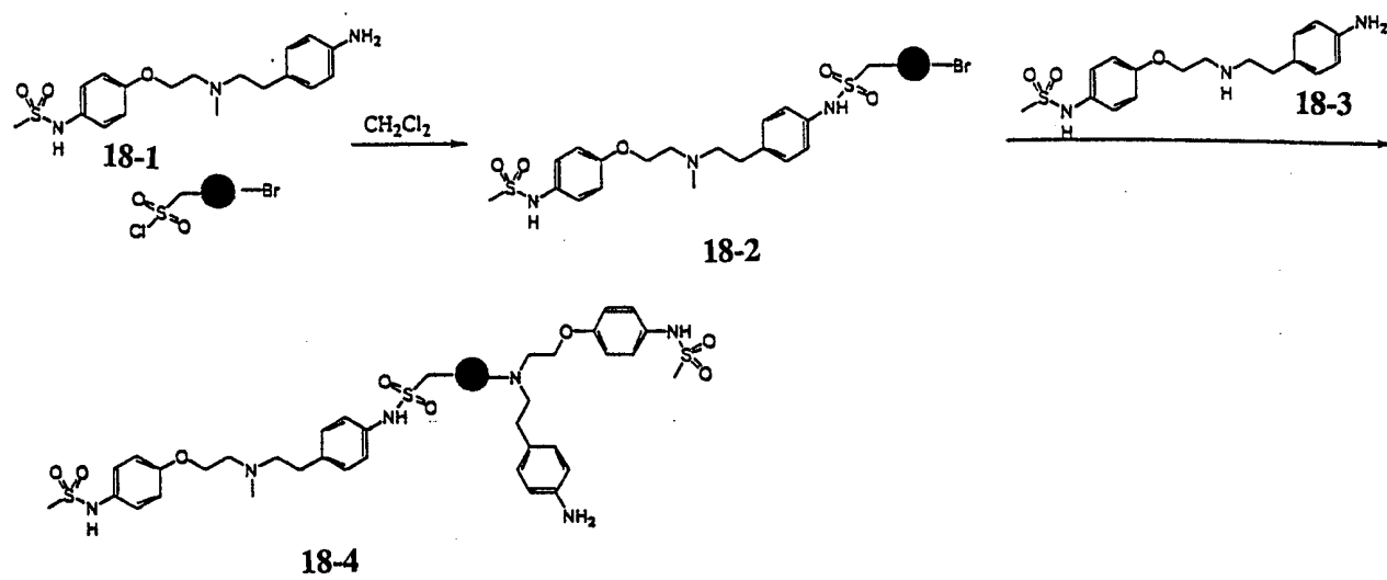
Figure 18. Assymmetric Linear Bivalent Compound
