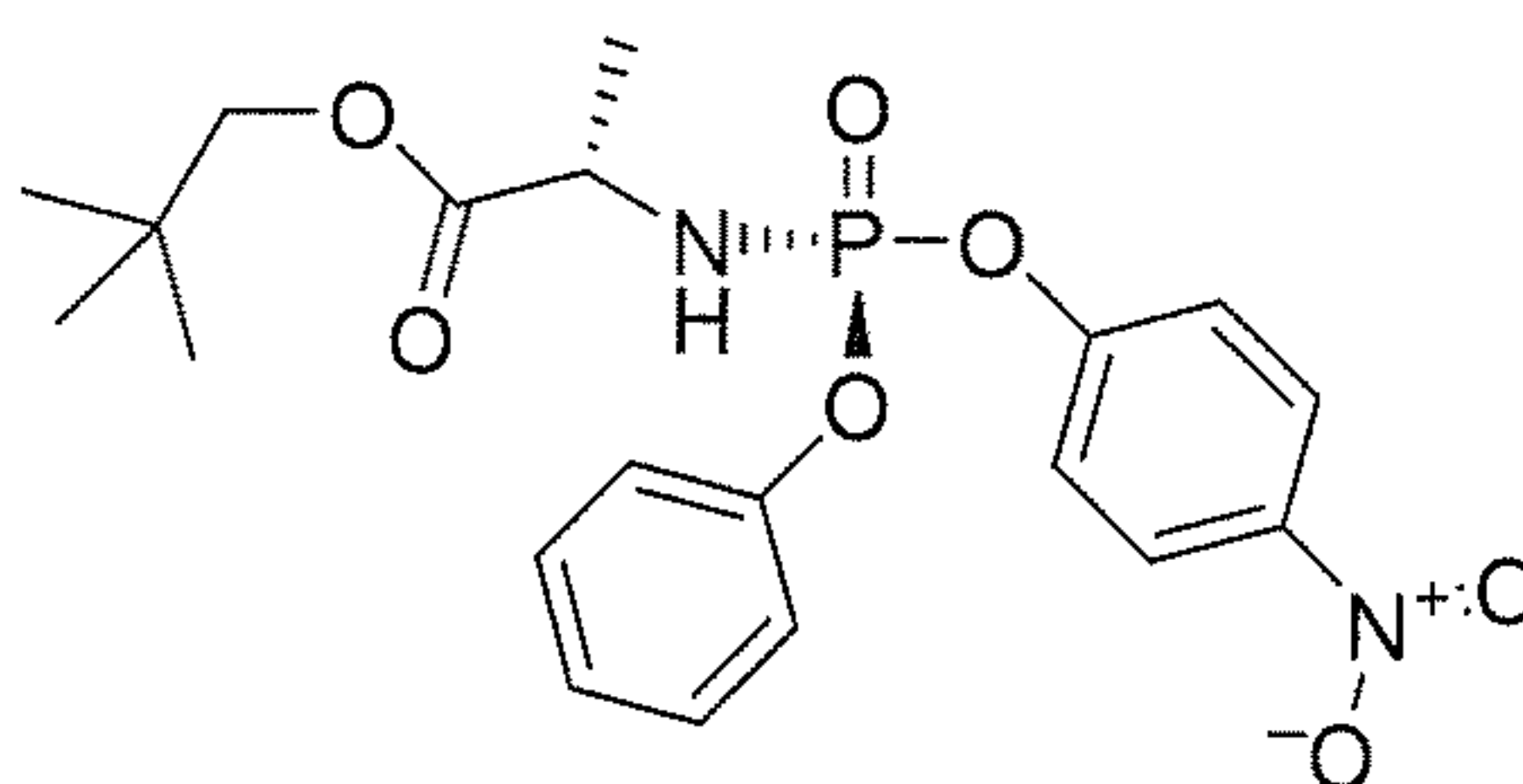
Compound 24
