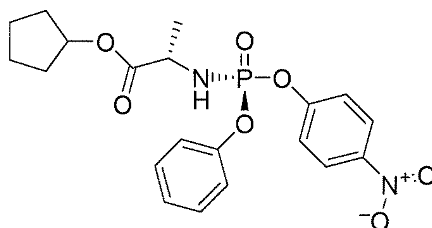
Compound 17
