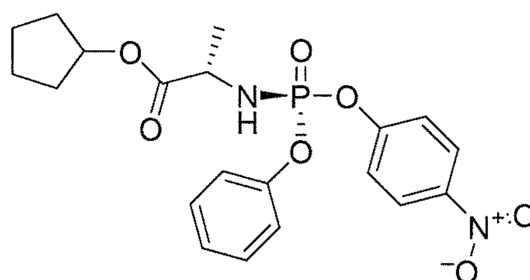
Compound 16
