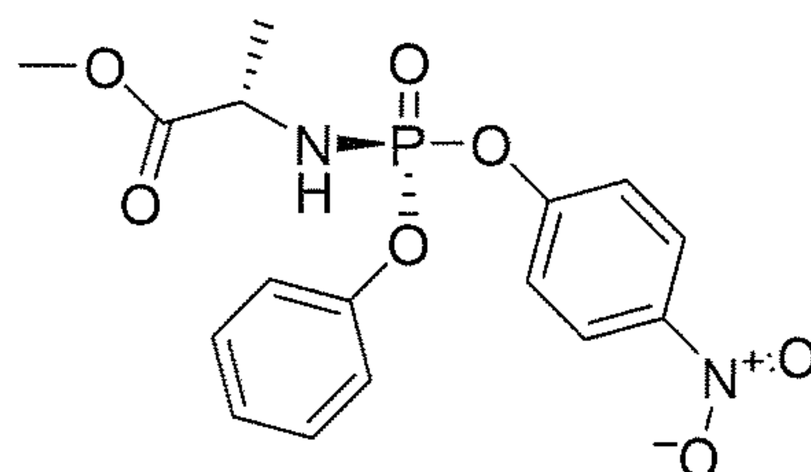
Compound 10
