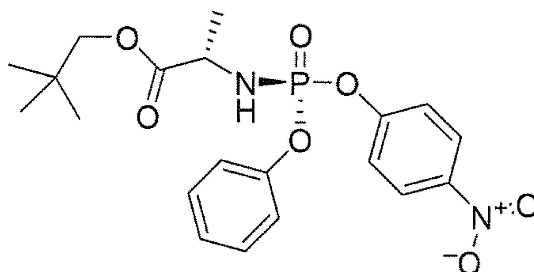
Compound 23
