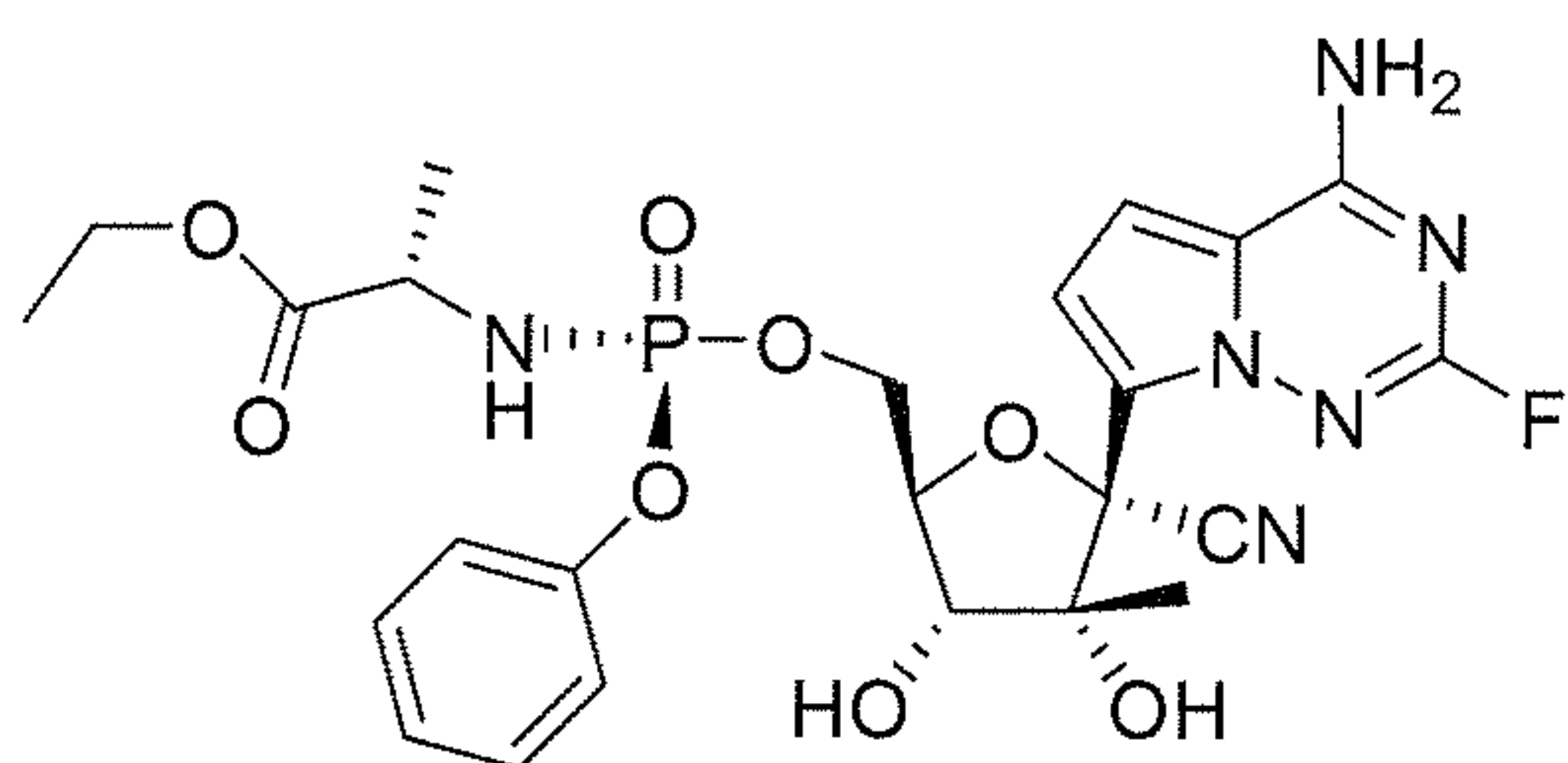
Compound 31
