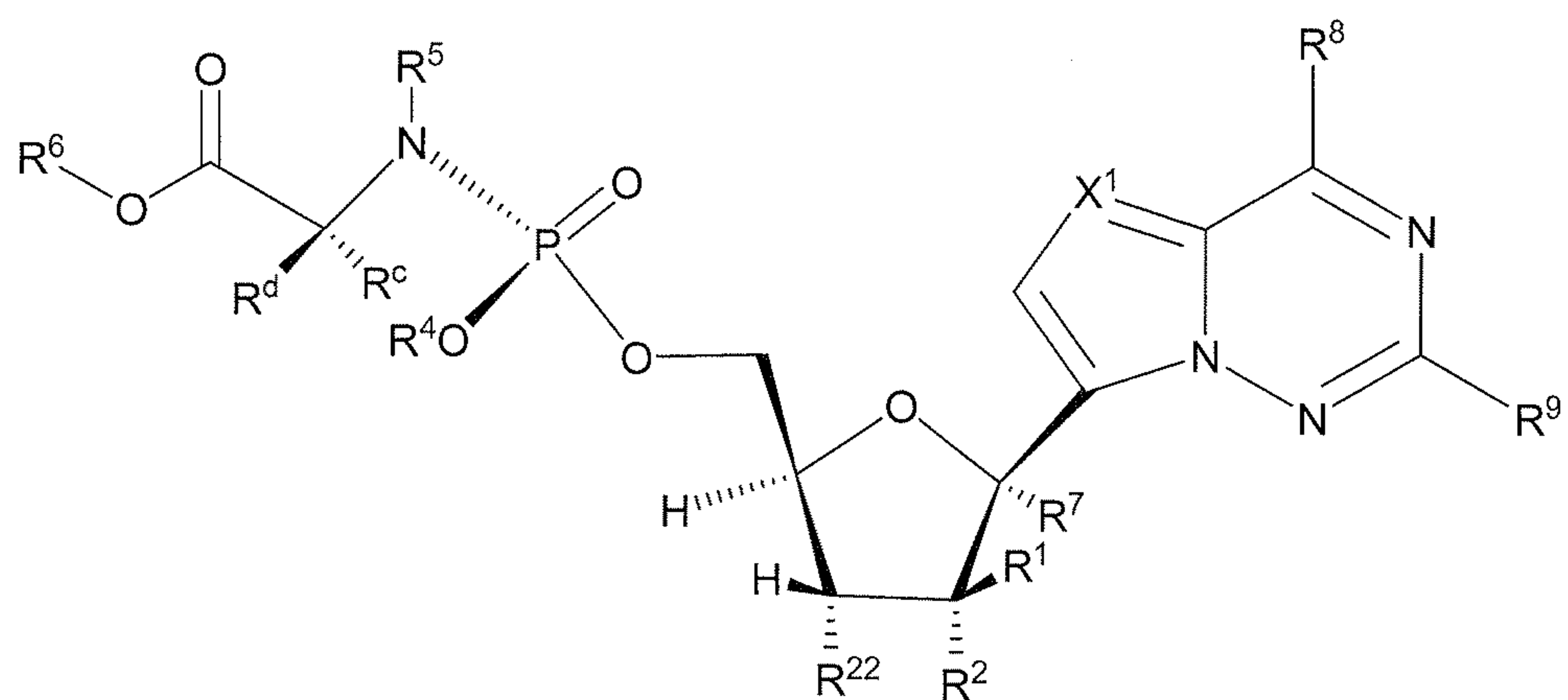
Formula VIa
