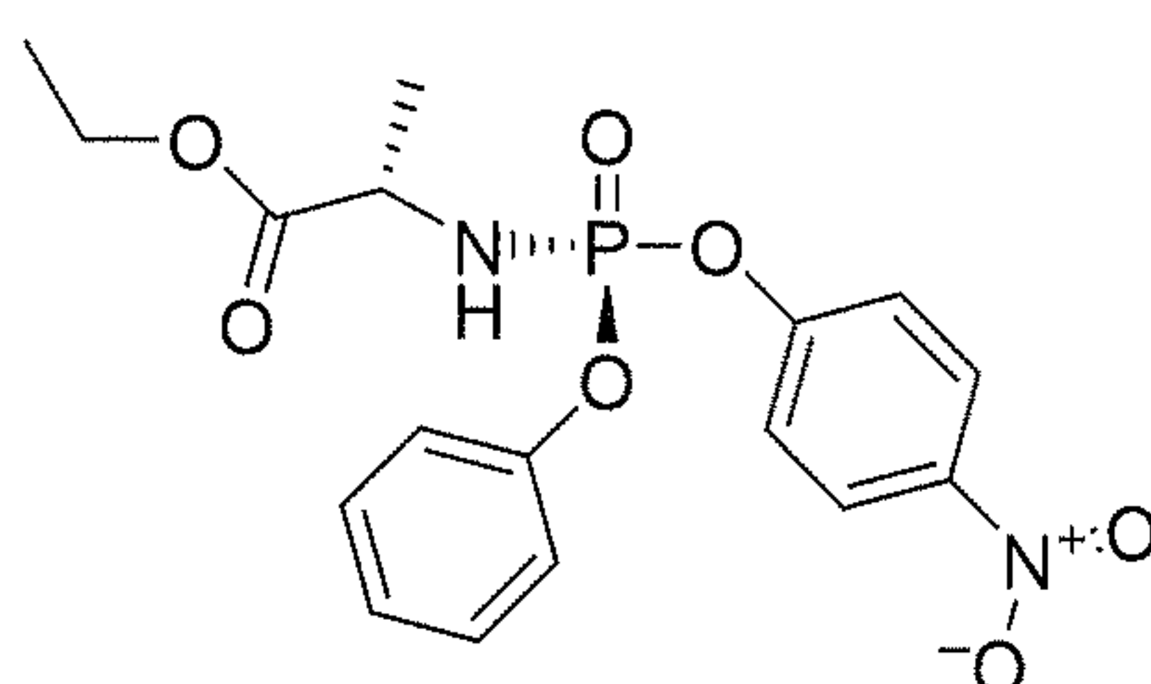
Compound 13
