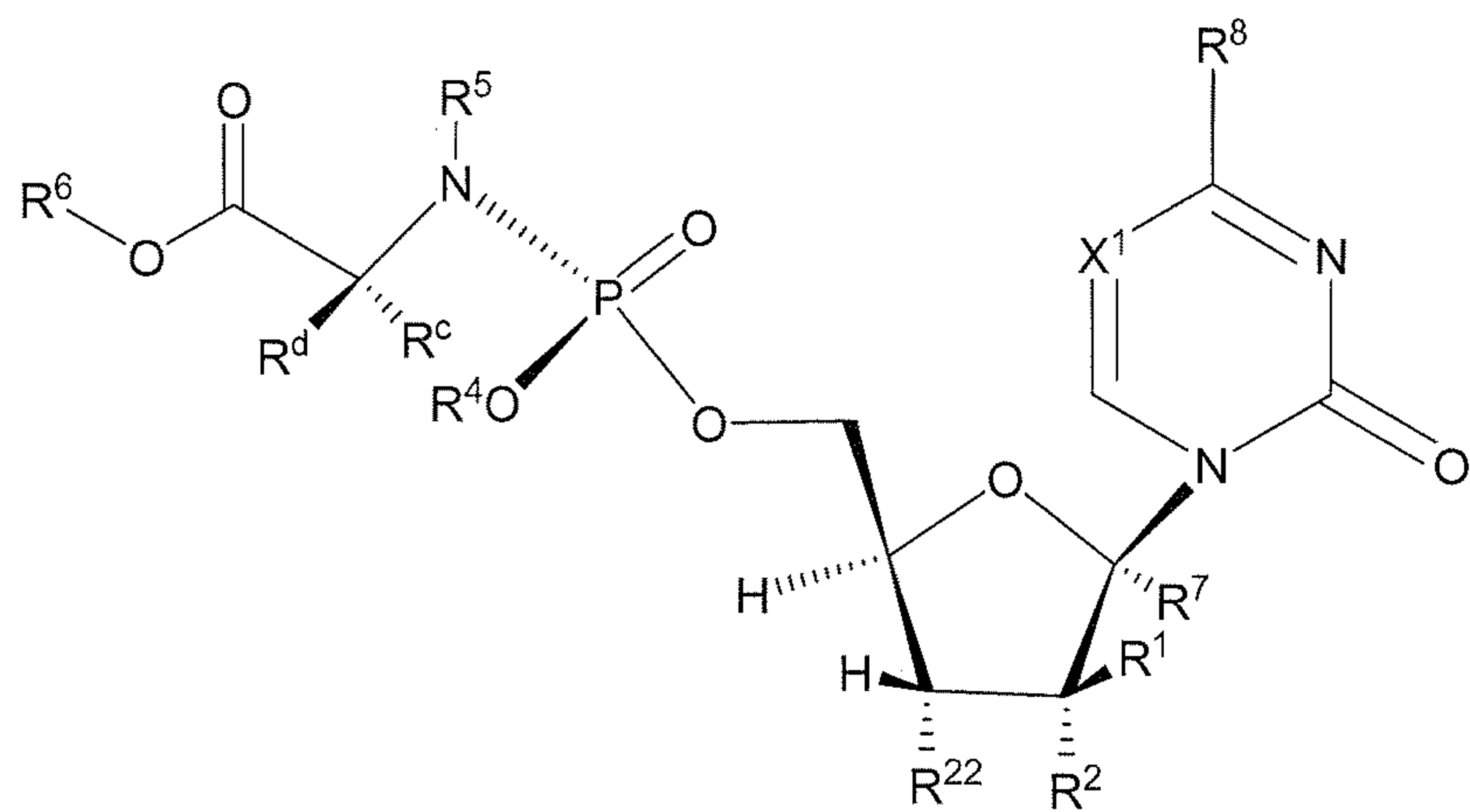
Formula XIIIa
