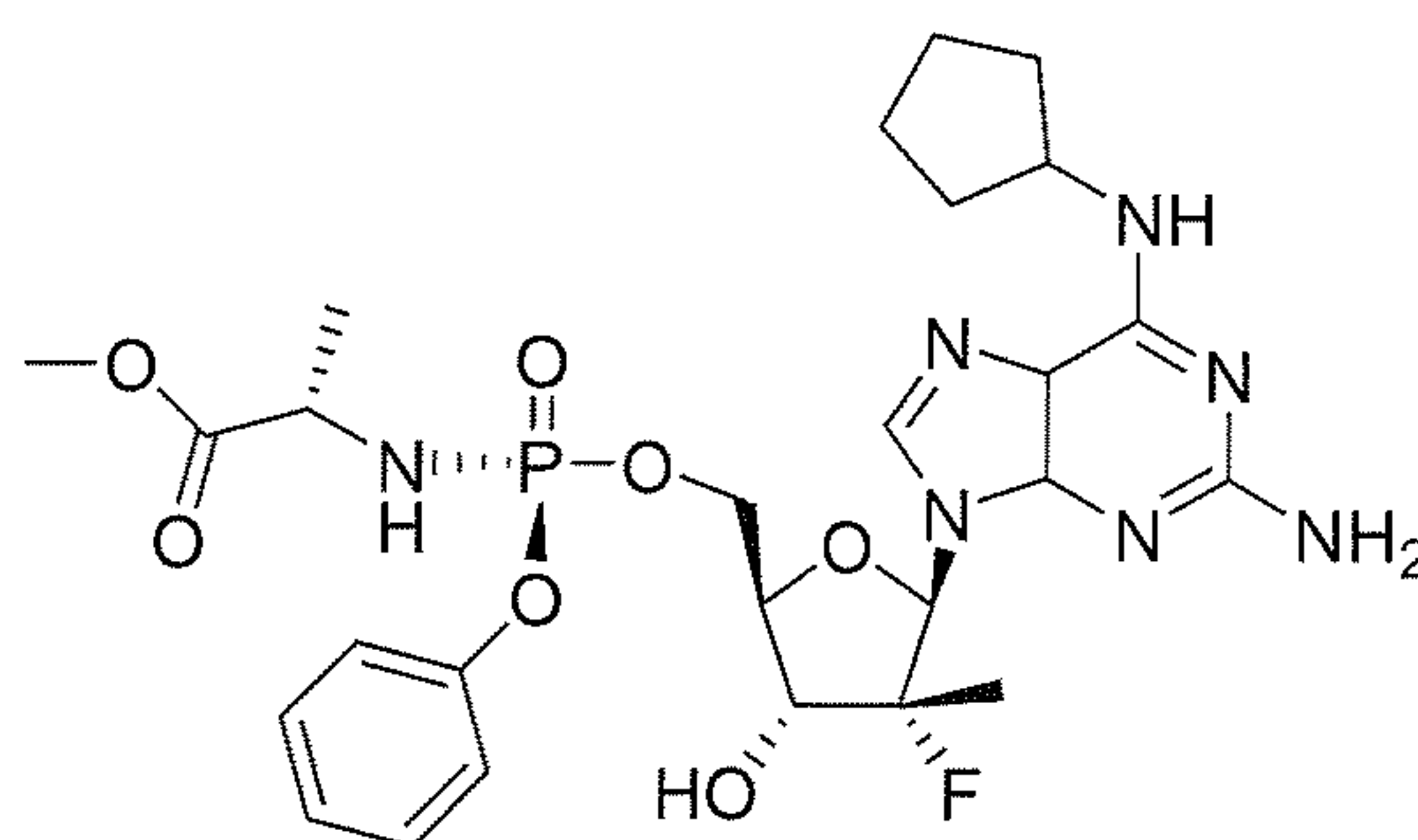
Compound 37
