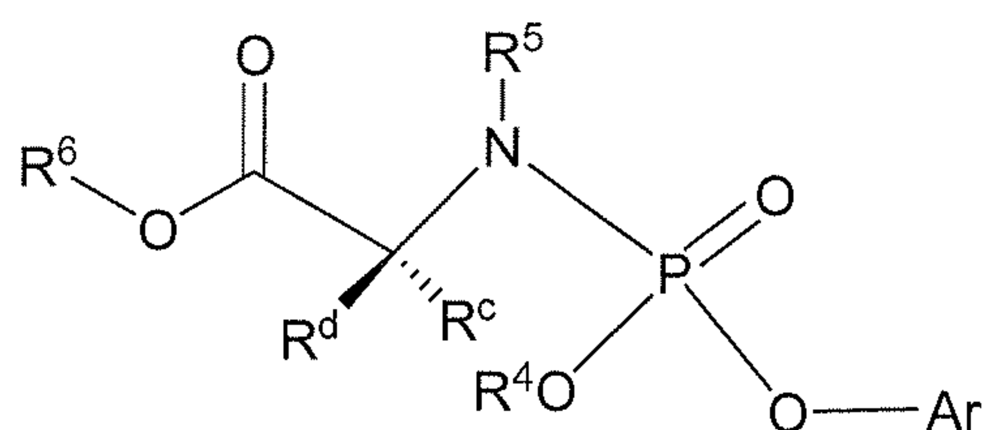
Formula VIII
