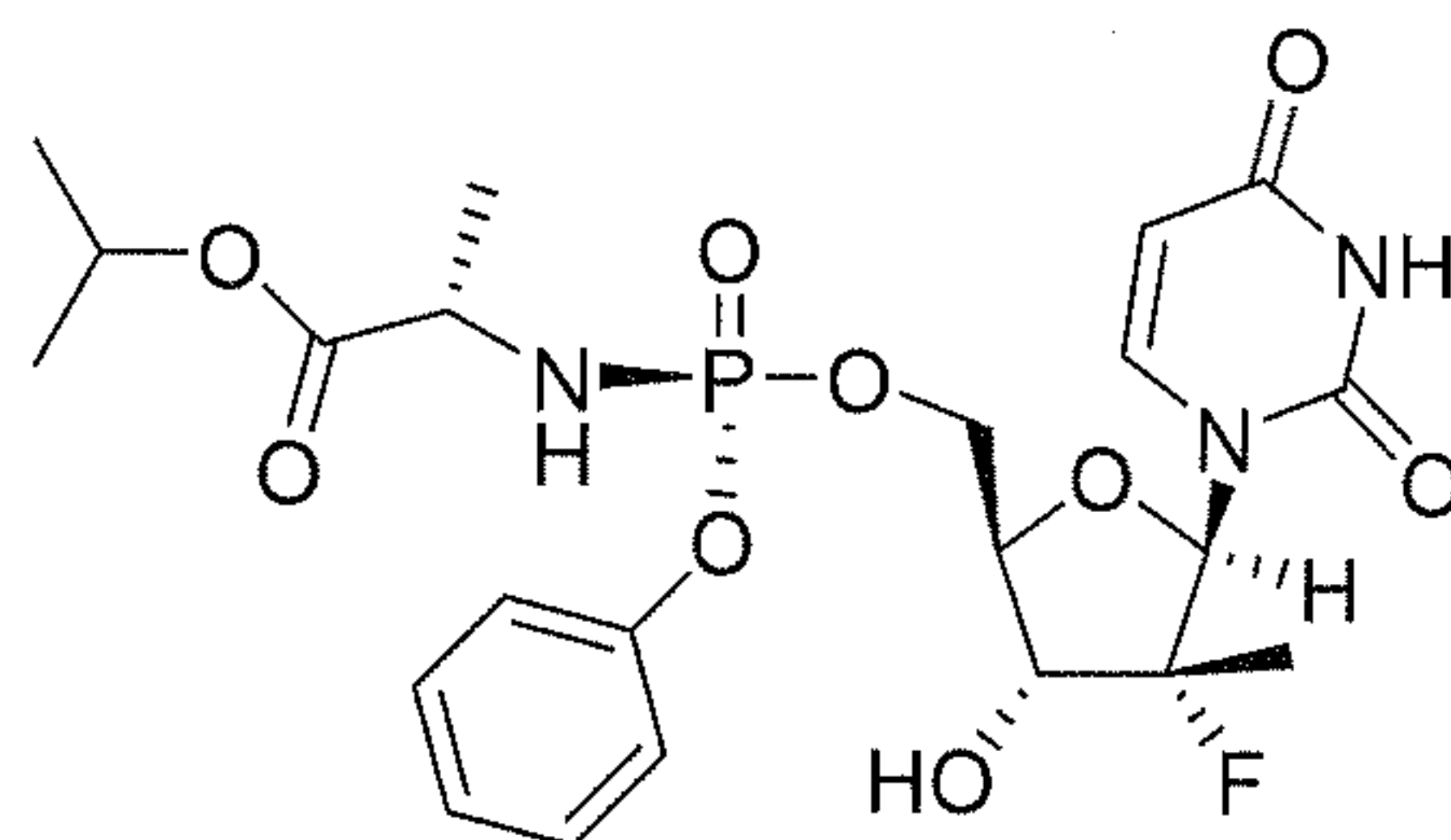
Compound 34
