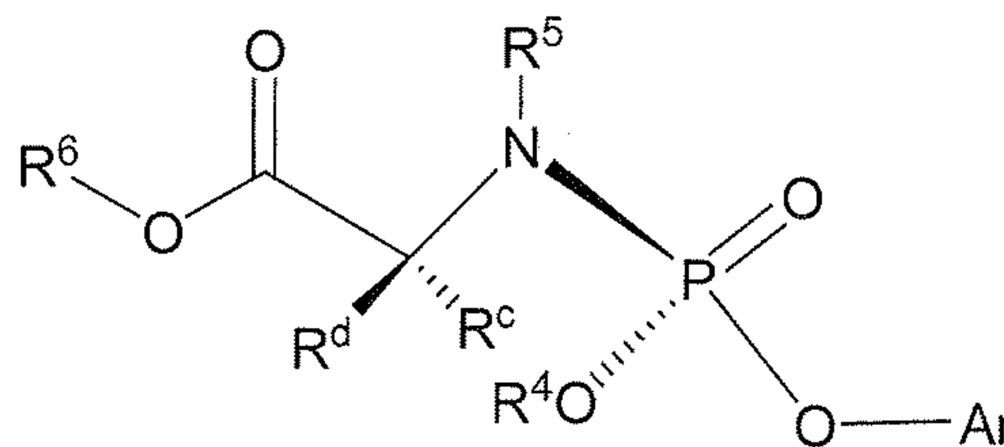
Formula IIIa
