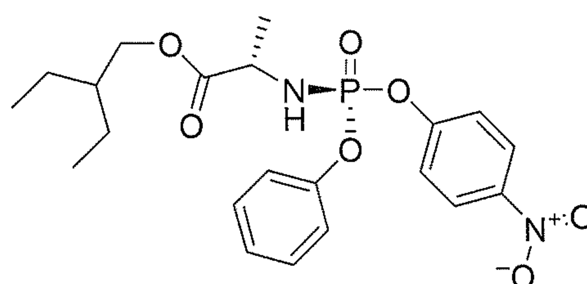
Compound 13
