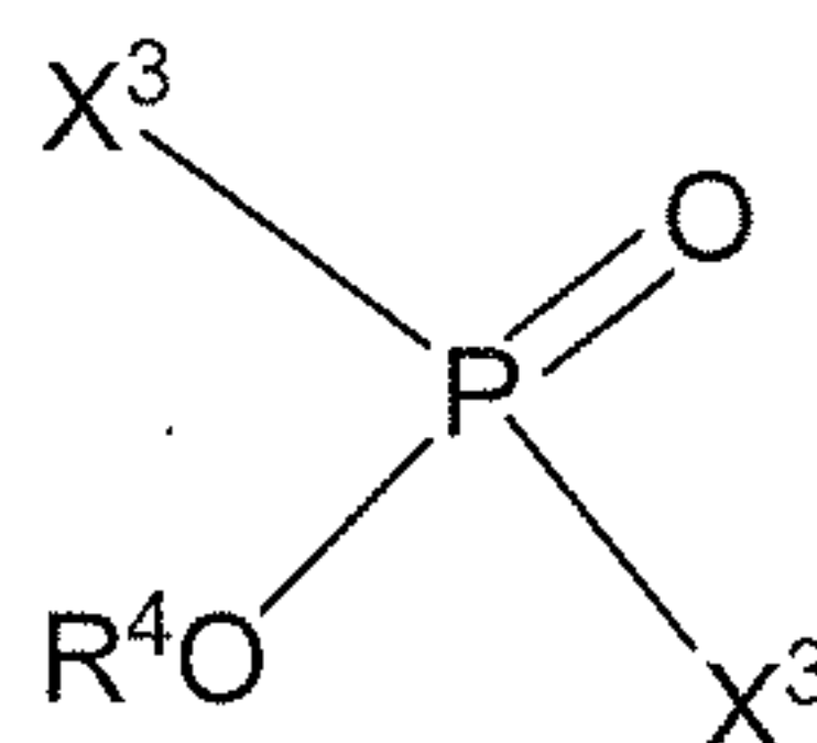
Formula X
