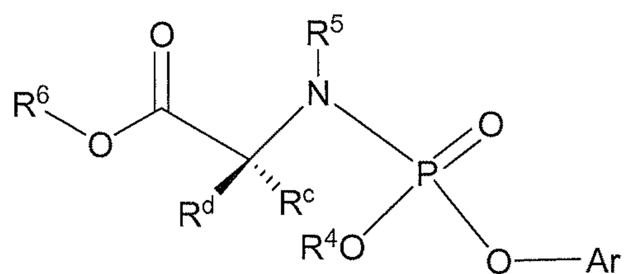
Formula VIII
