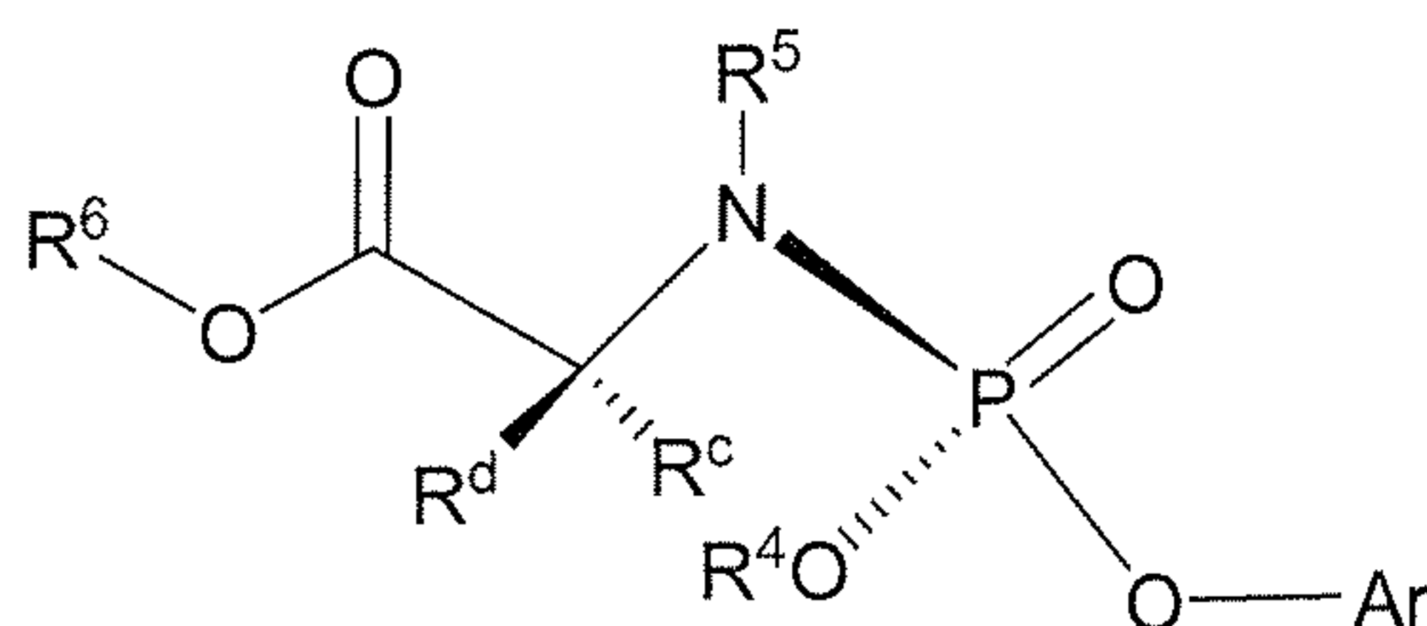
Formula IIIa
