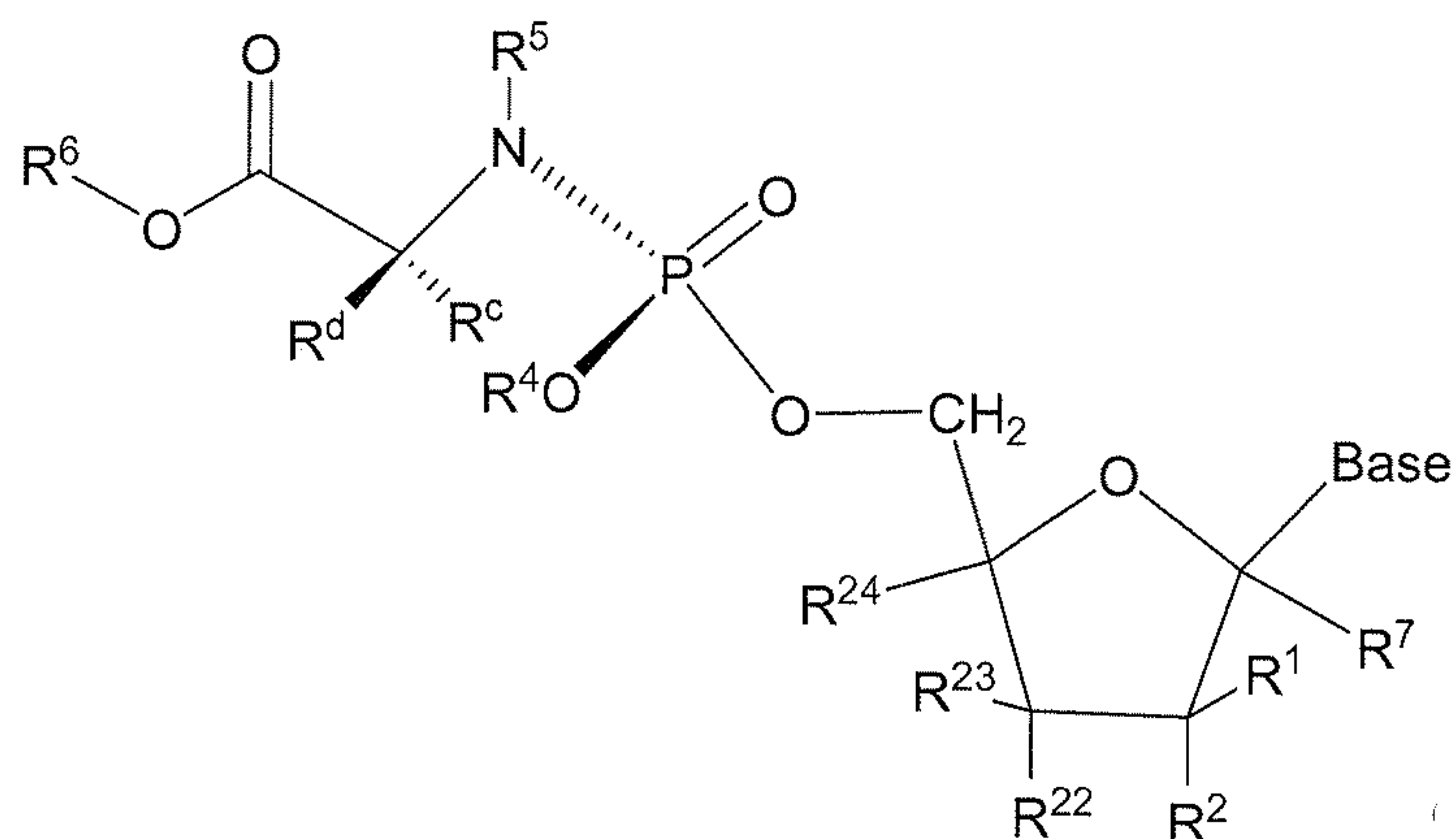
Formula Ia
