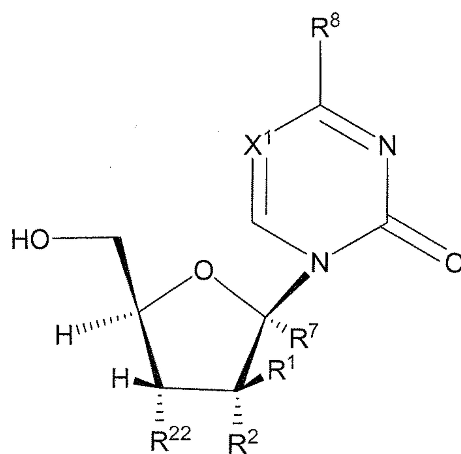
Formula XIV
