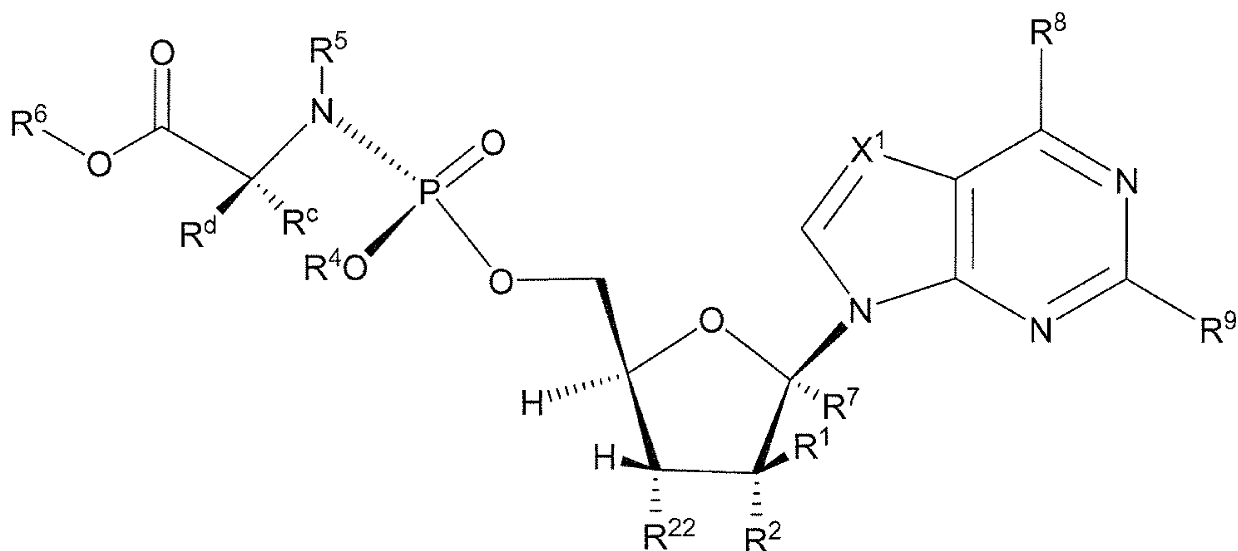
Formula XIa
