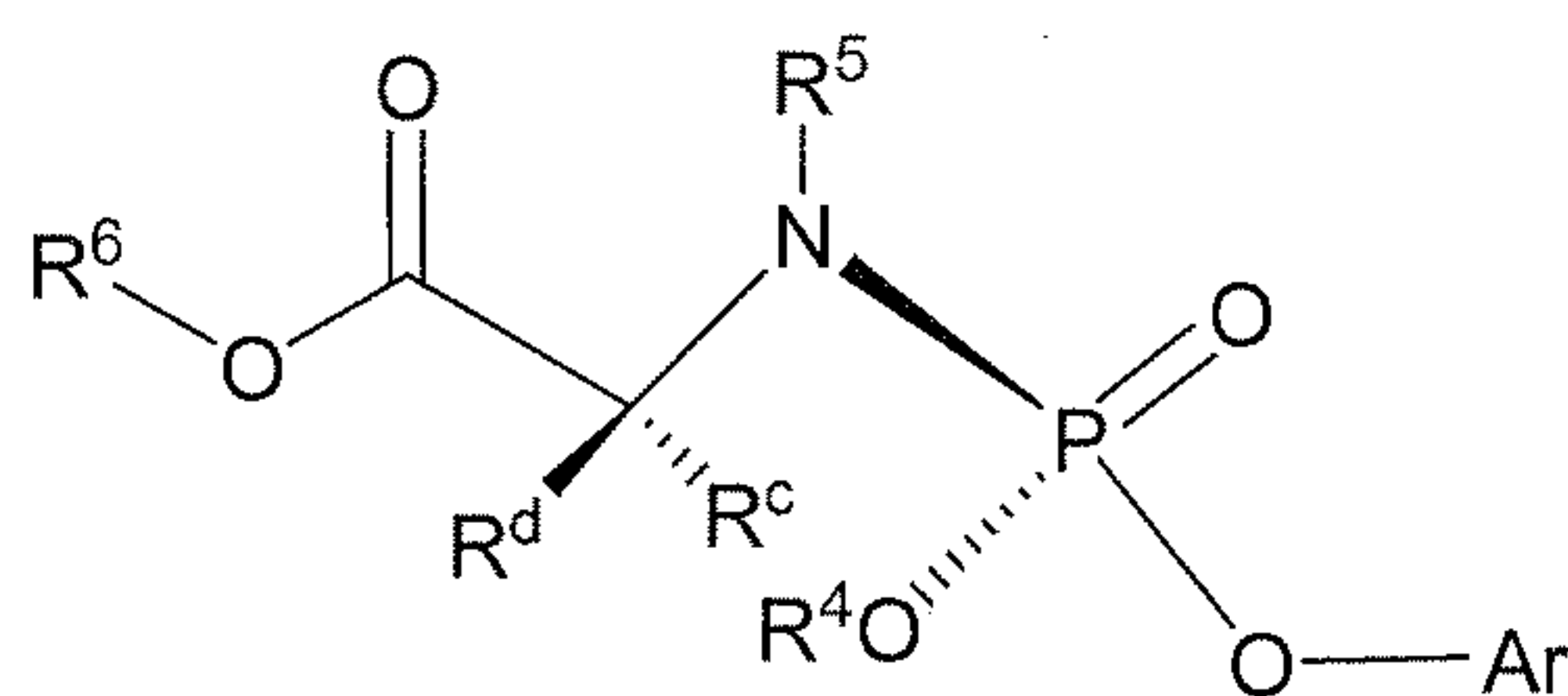
Formula IIIa
