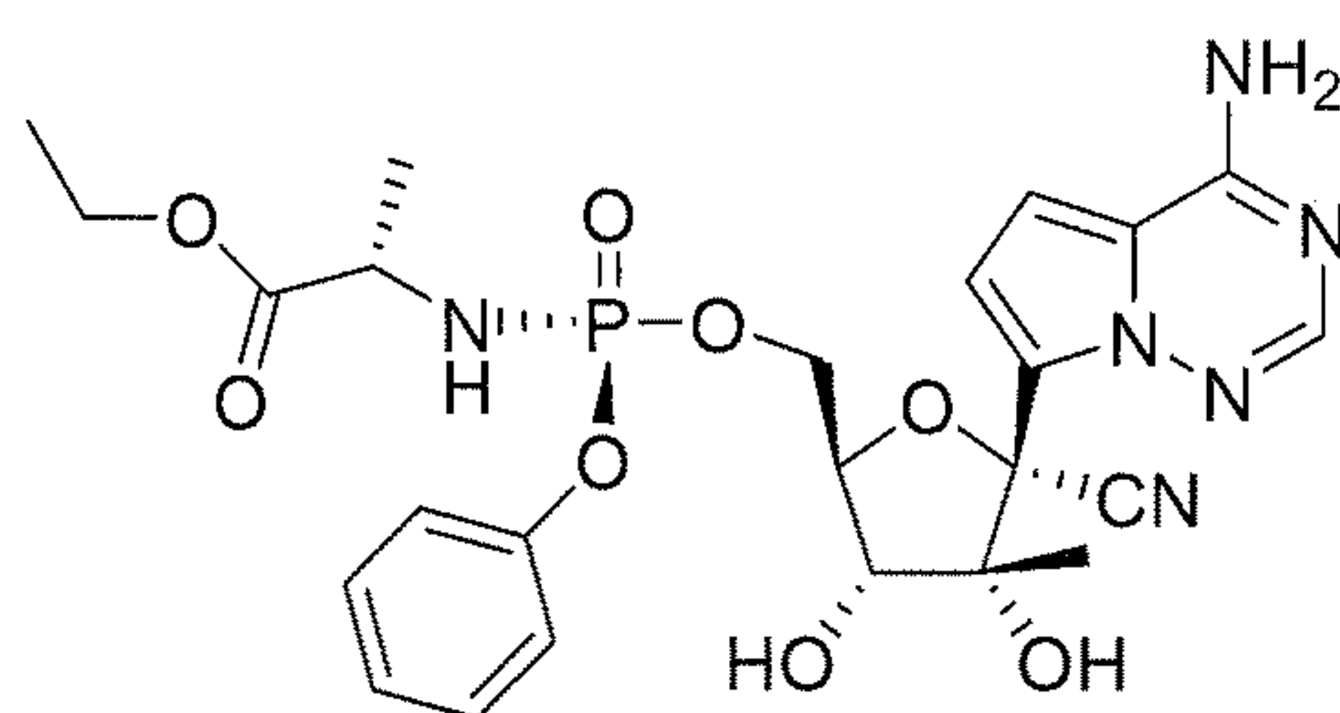
Compound 25
