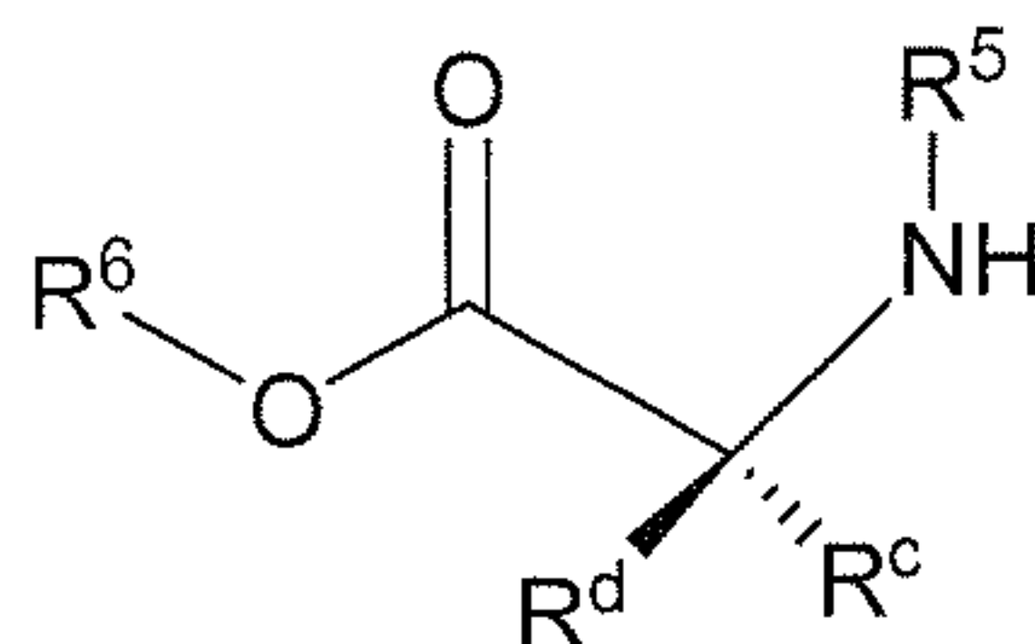
Formula IX
