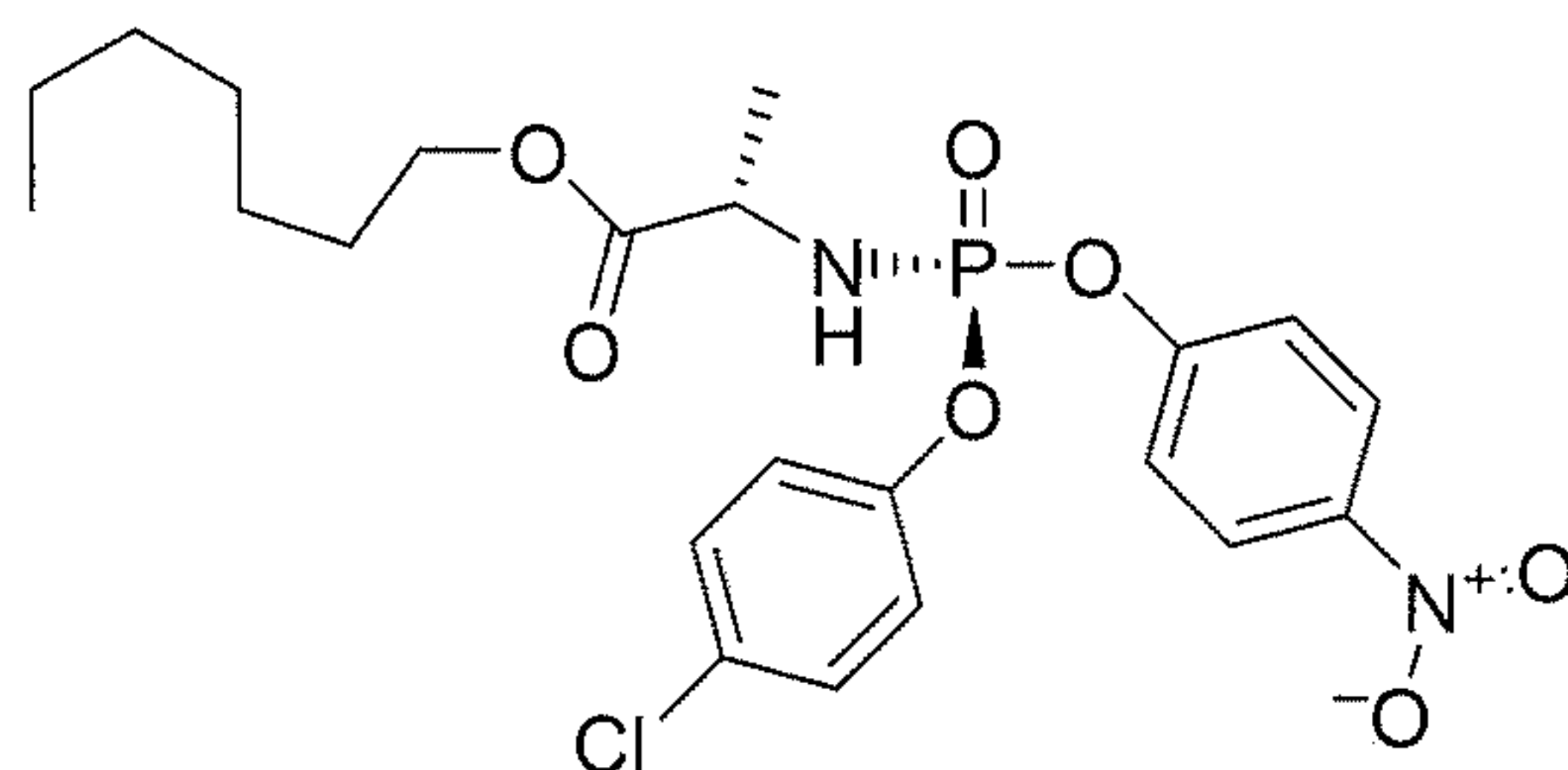
Compound 19
