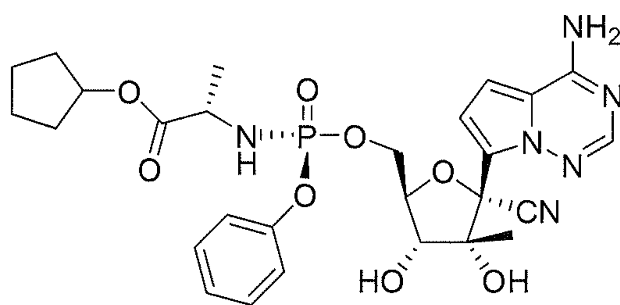
Compound 27
