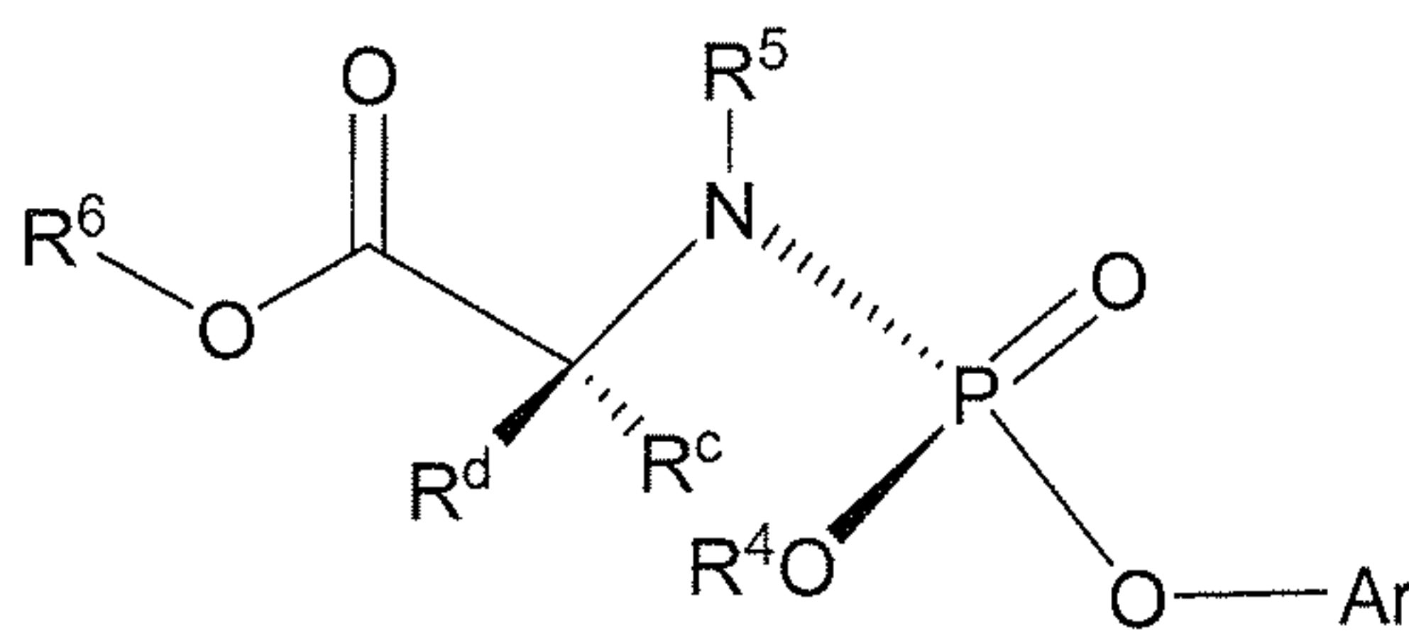
Formula IIIb
