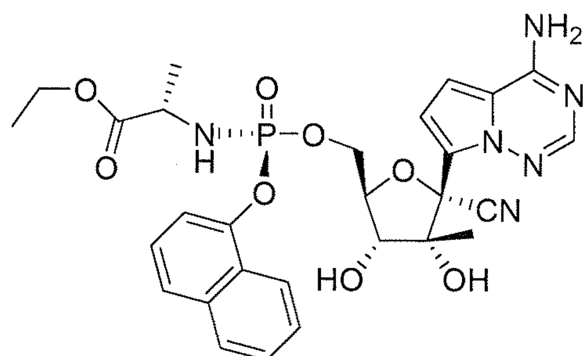
Compound 29
