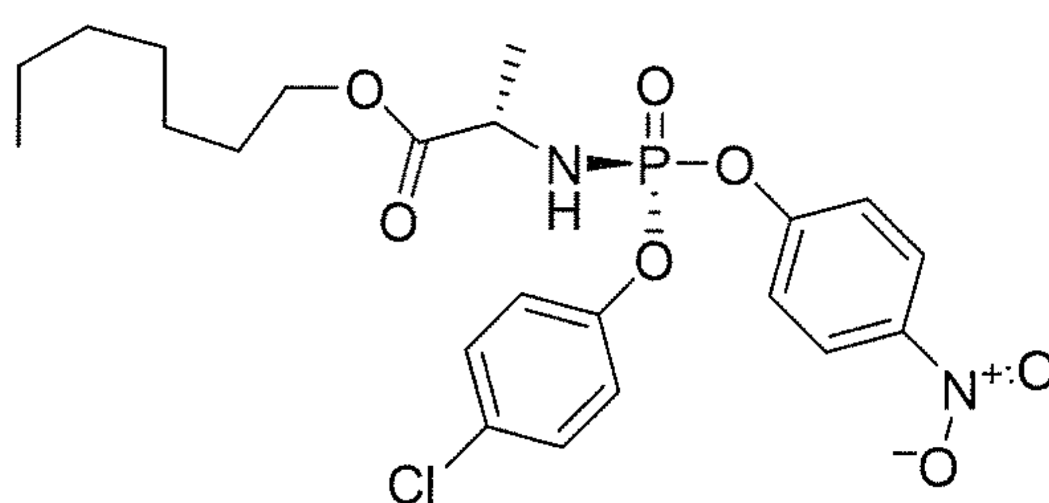
Compound 18
