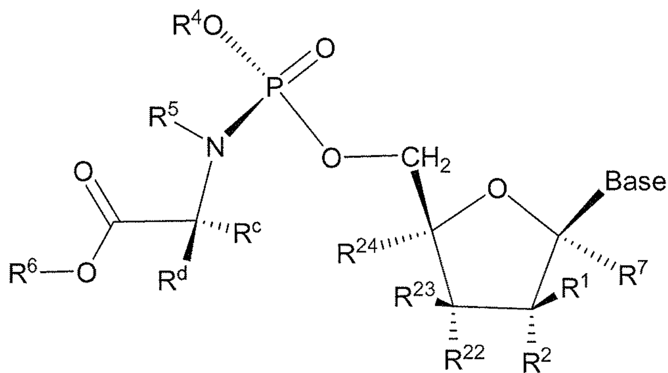
Formula IVb
