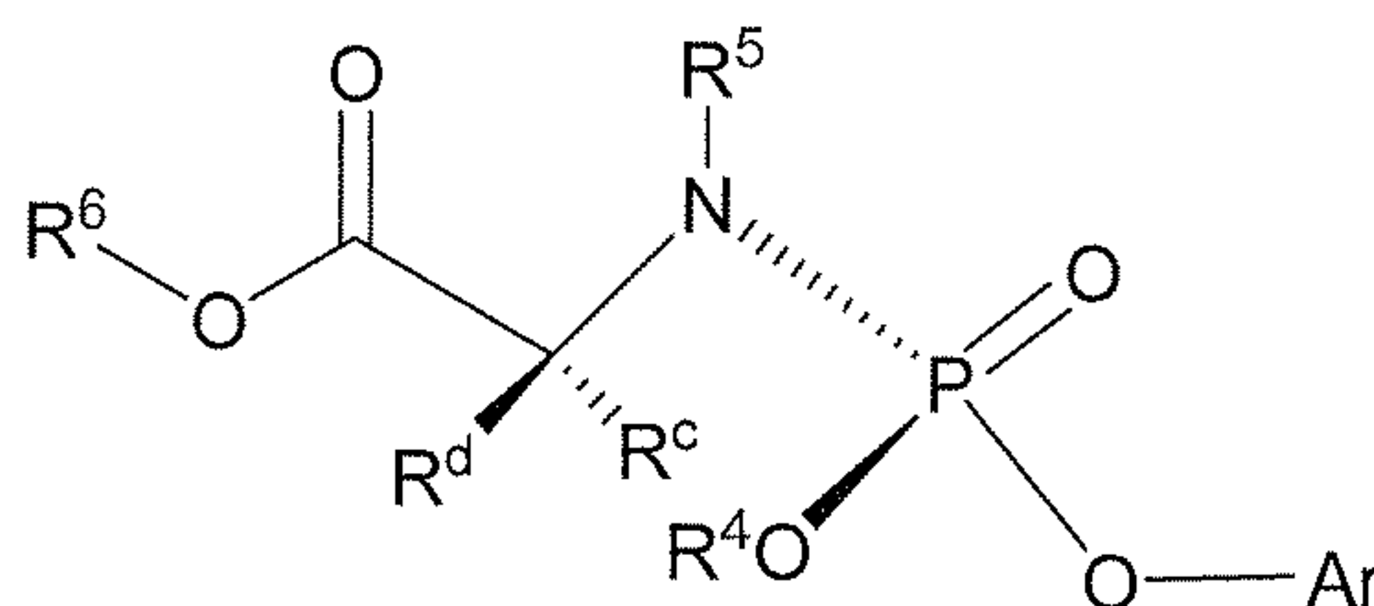
Formula IIIb
