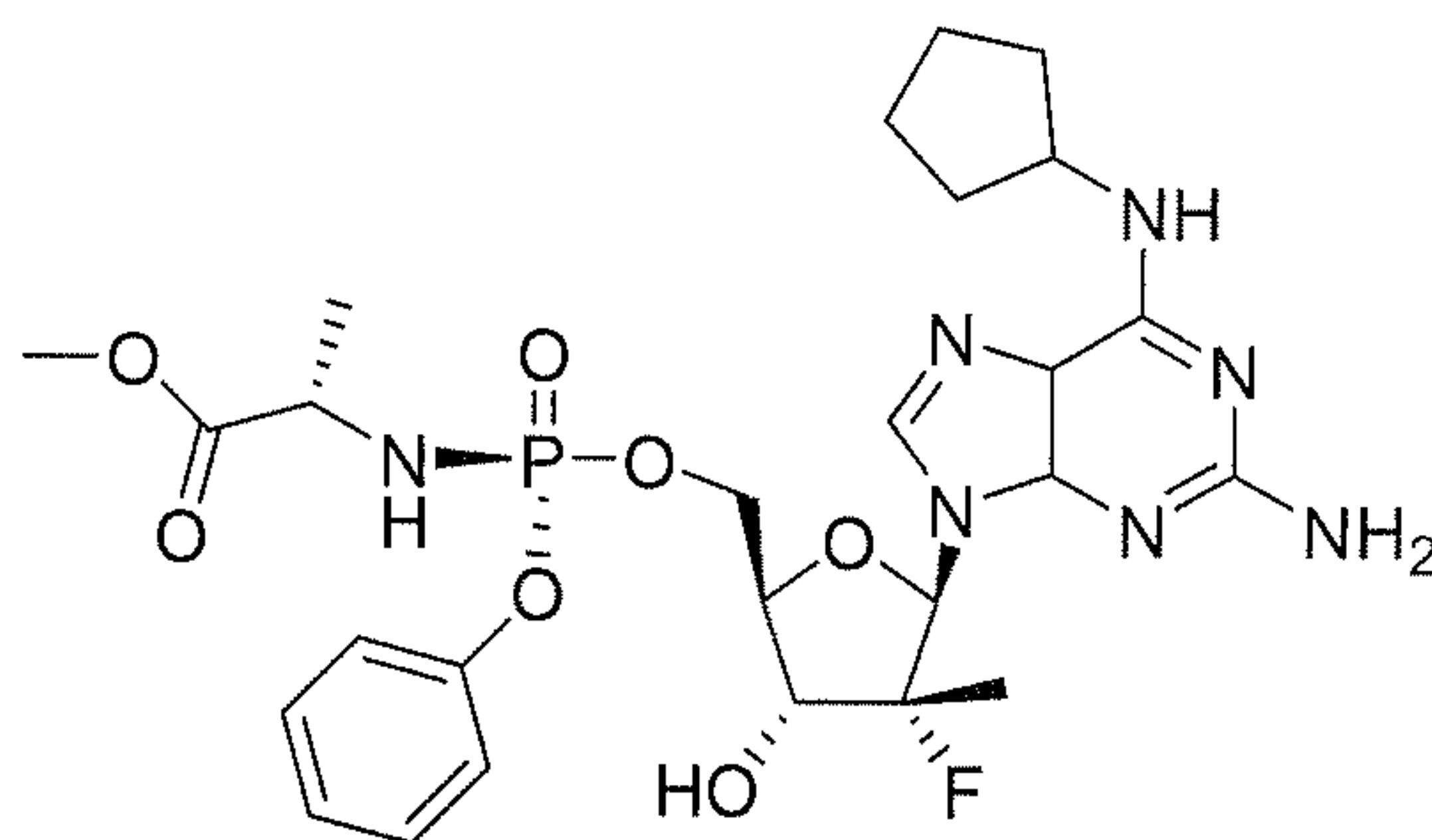
Compound 38
