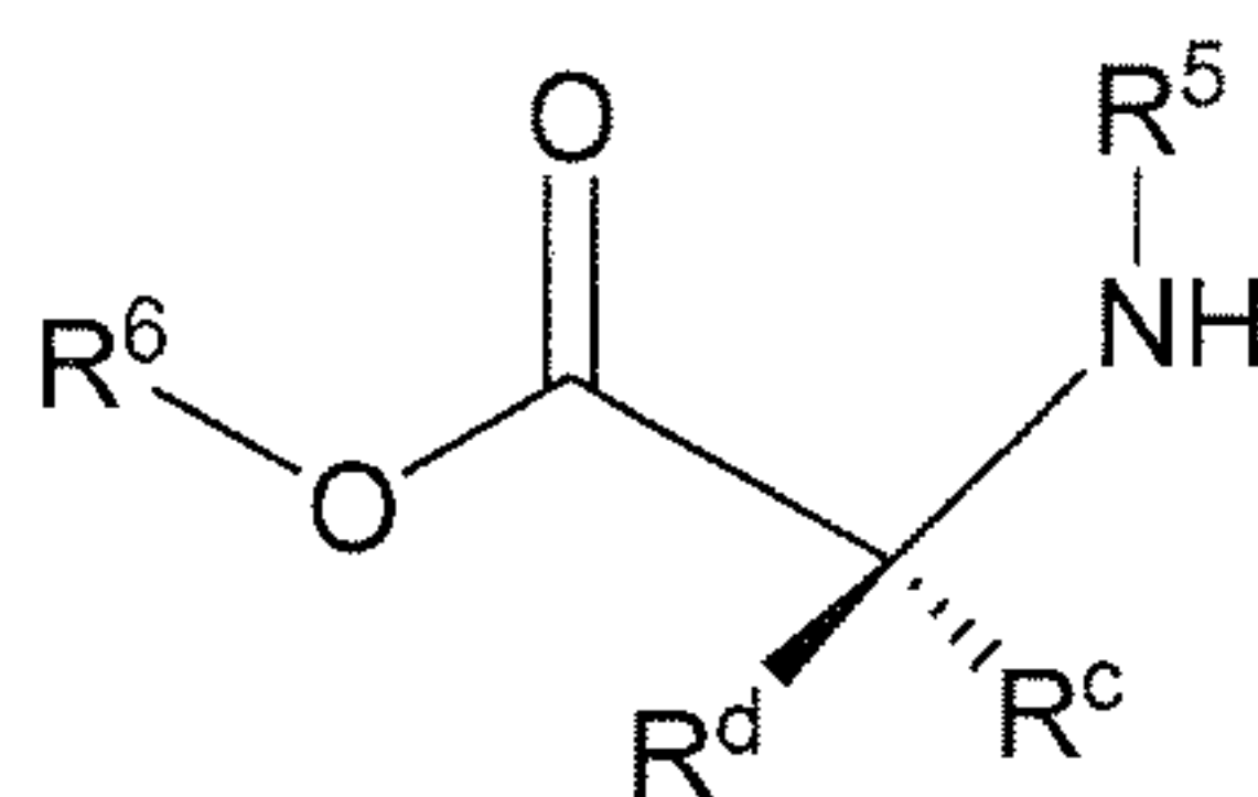
Formula IX
