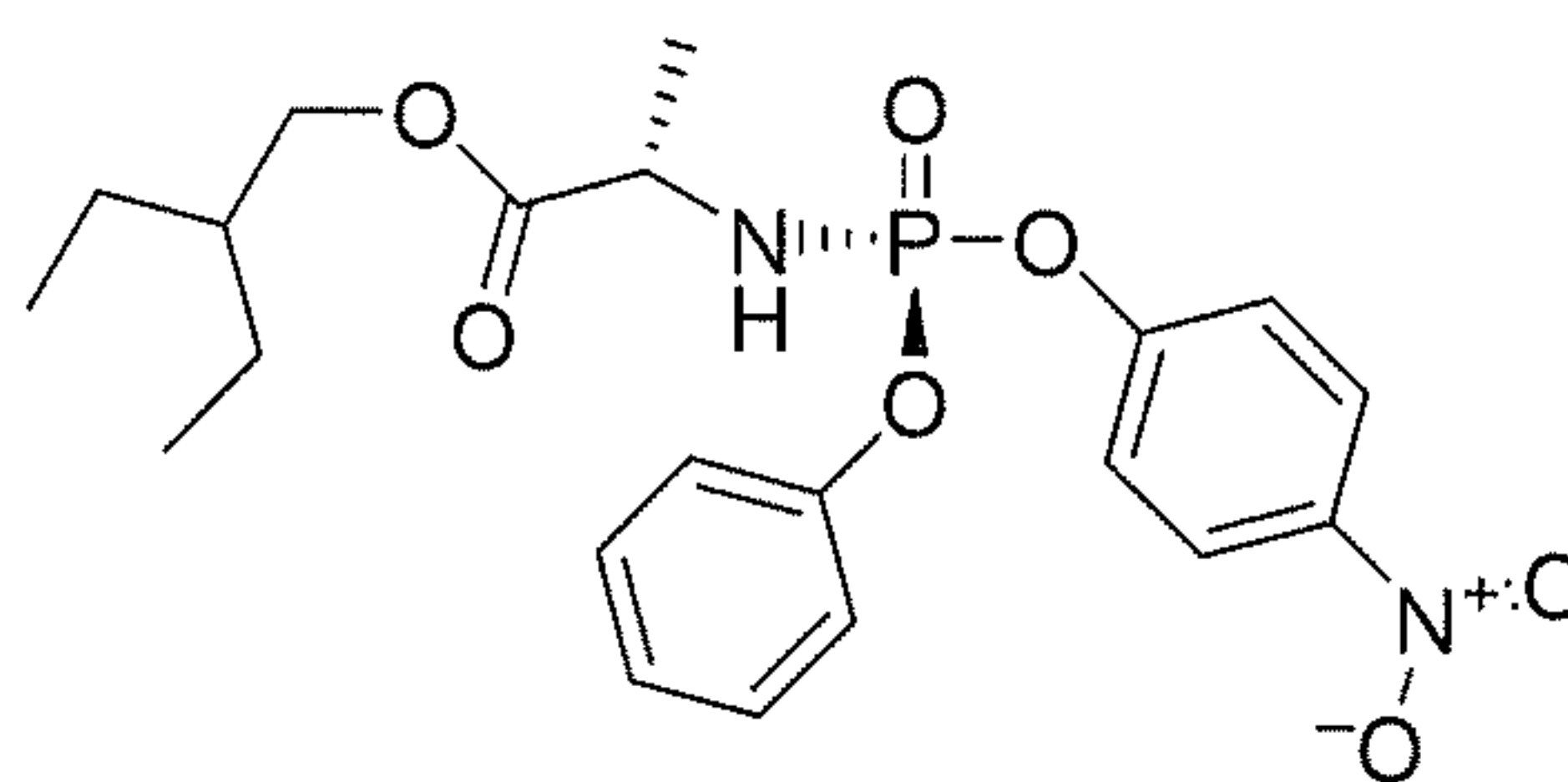
Compound 15
