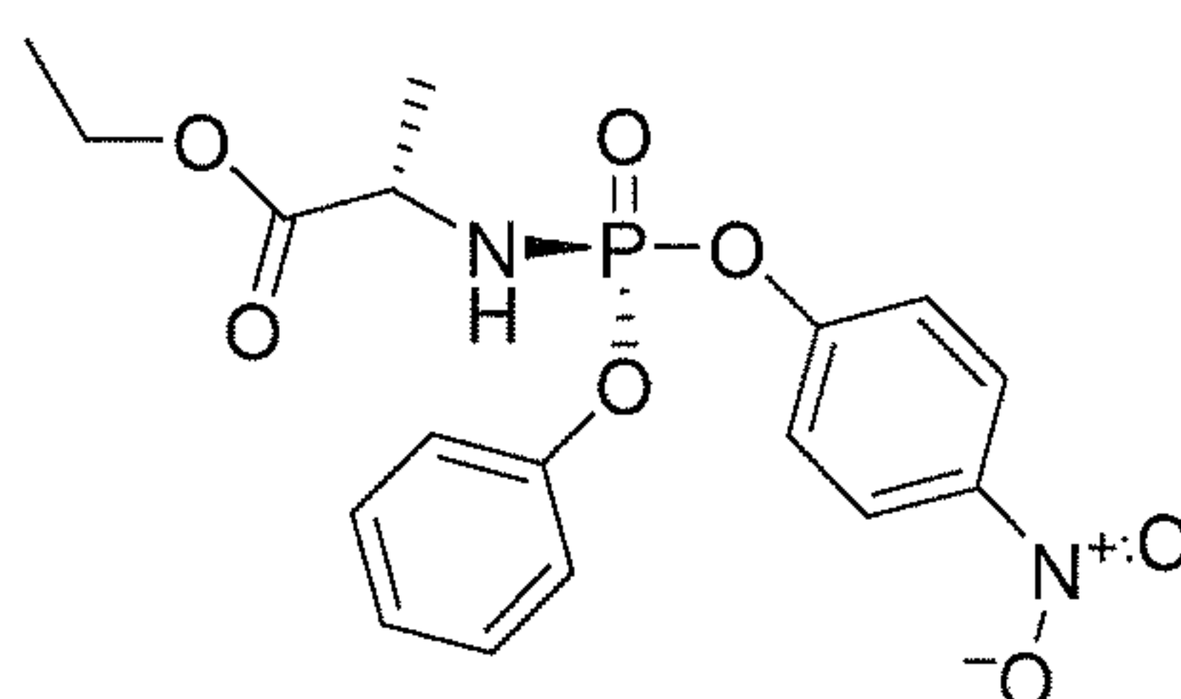
Compound 12
