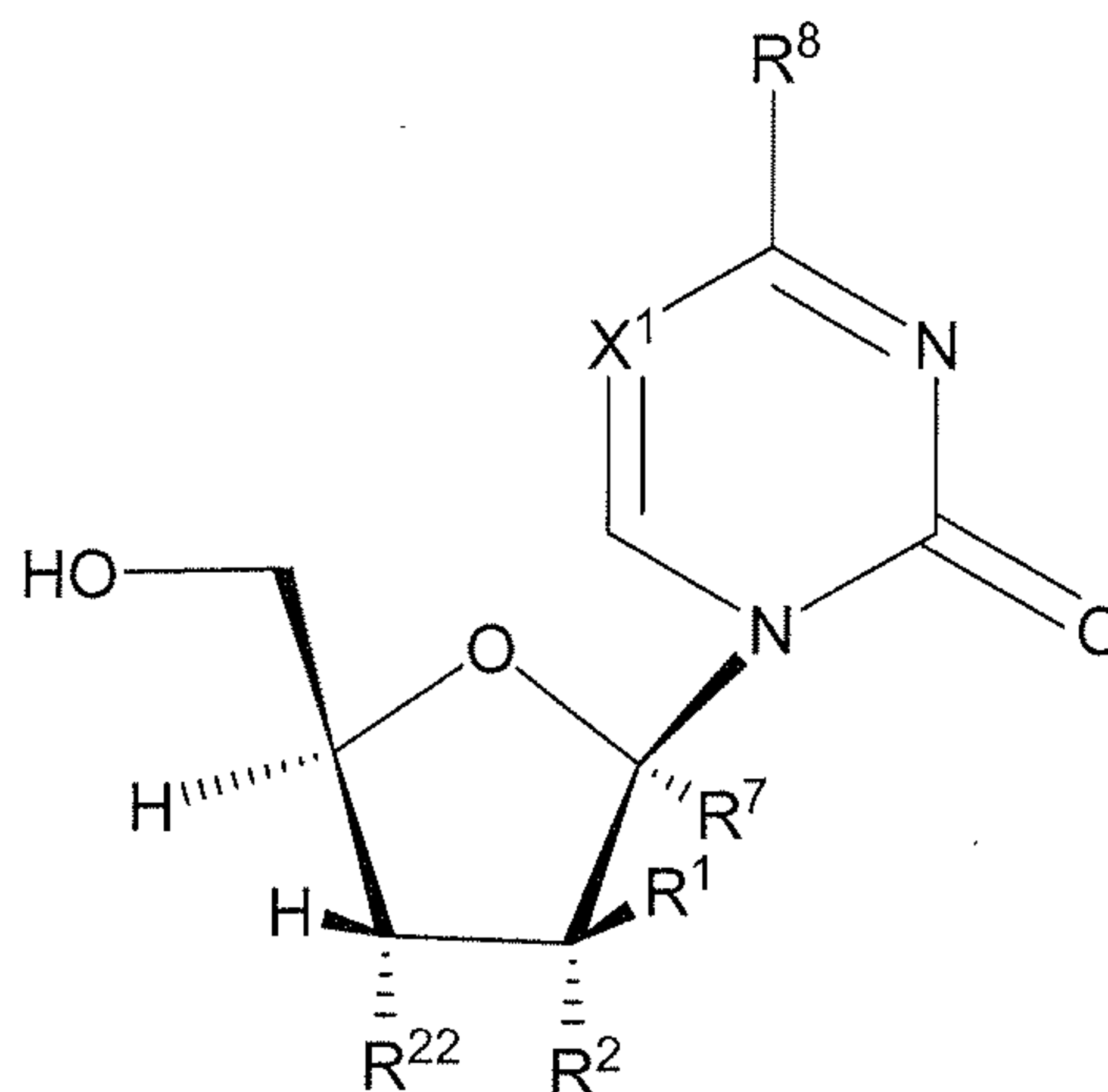
Formula XIV
