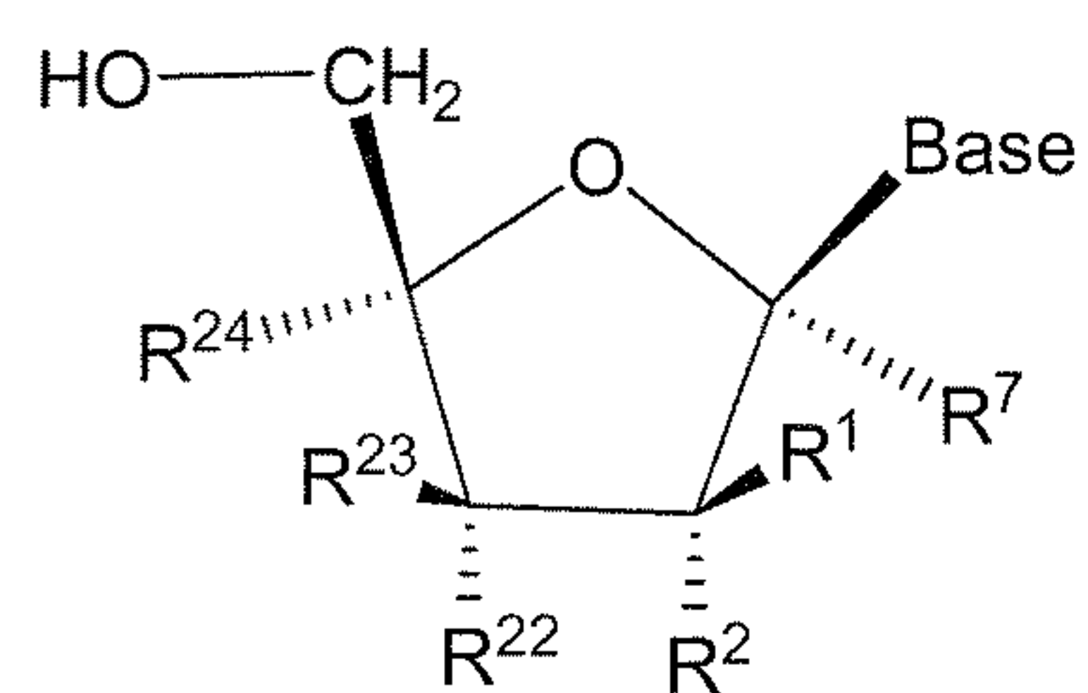
Formula V
