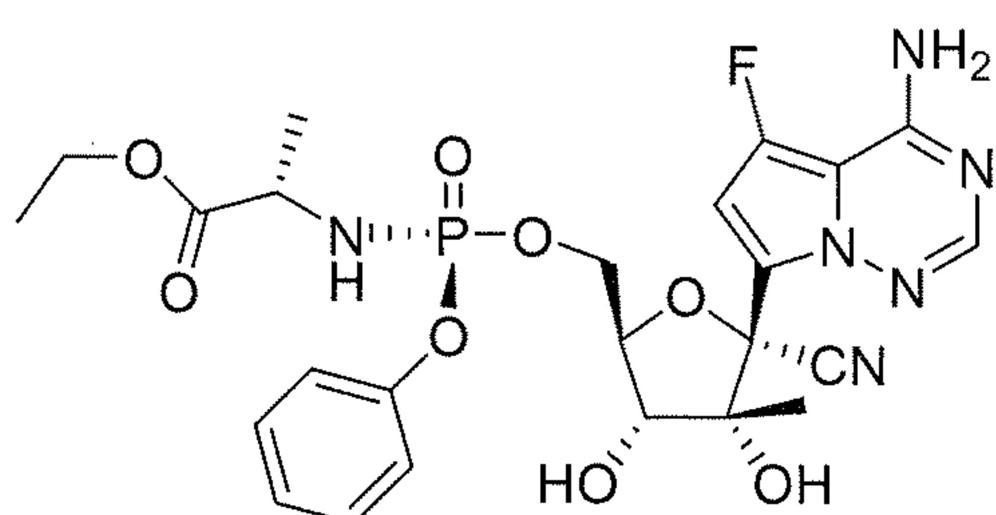
Compound 30
