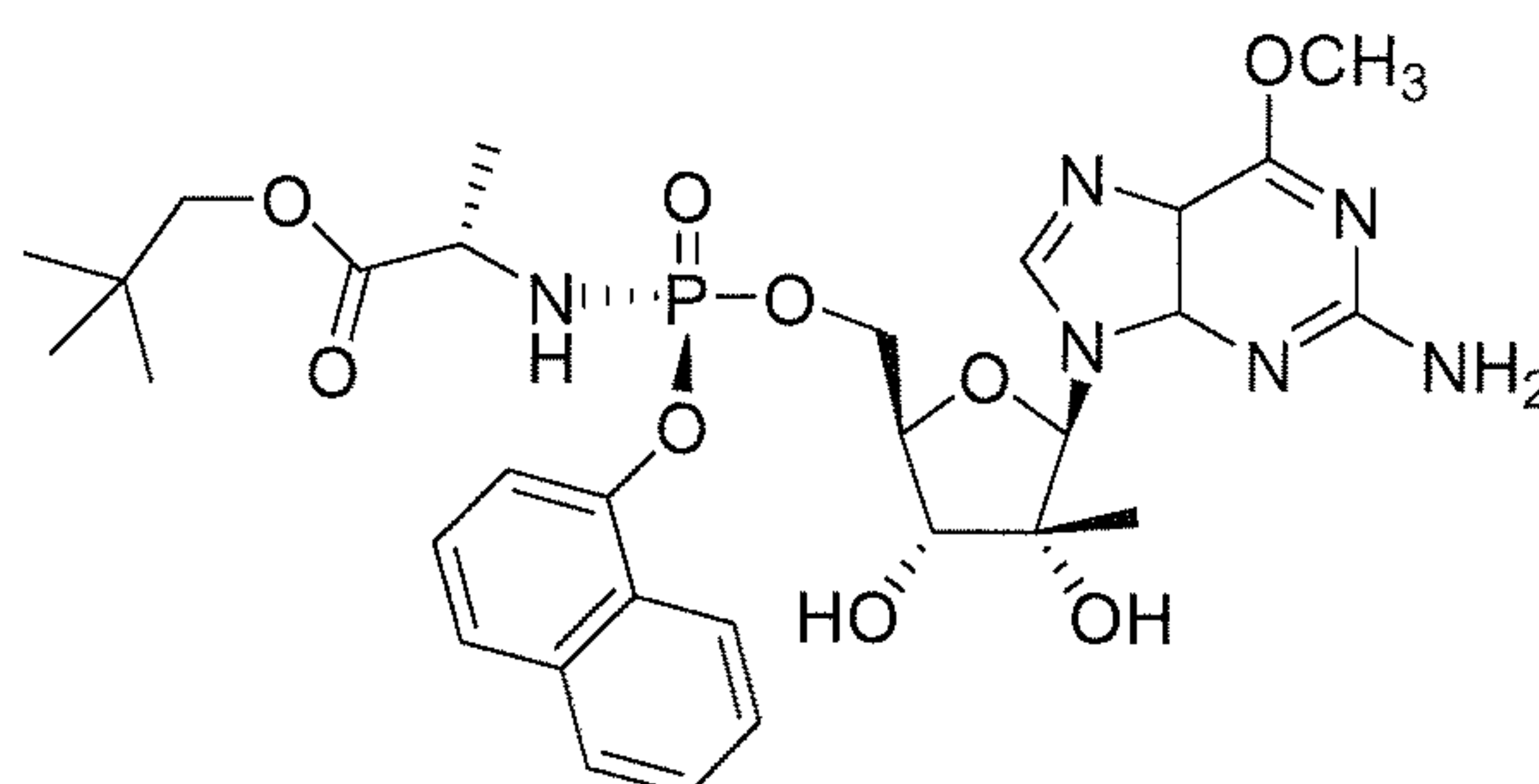
Compound 35
