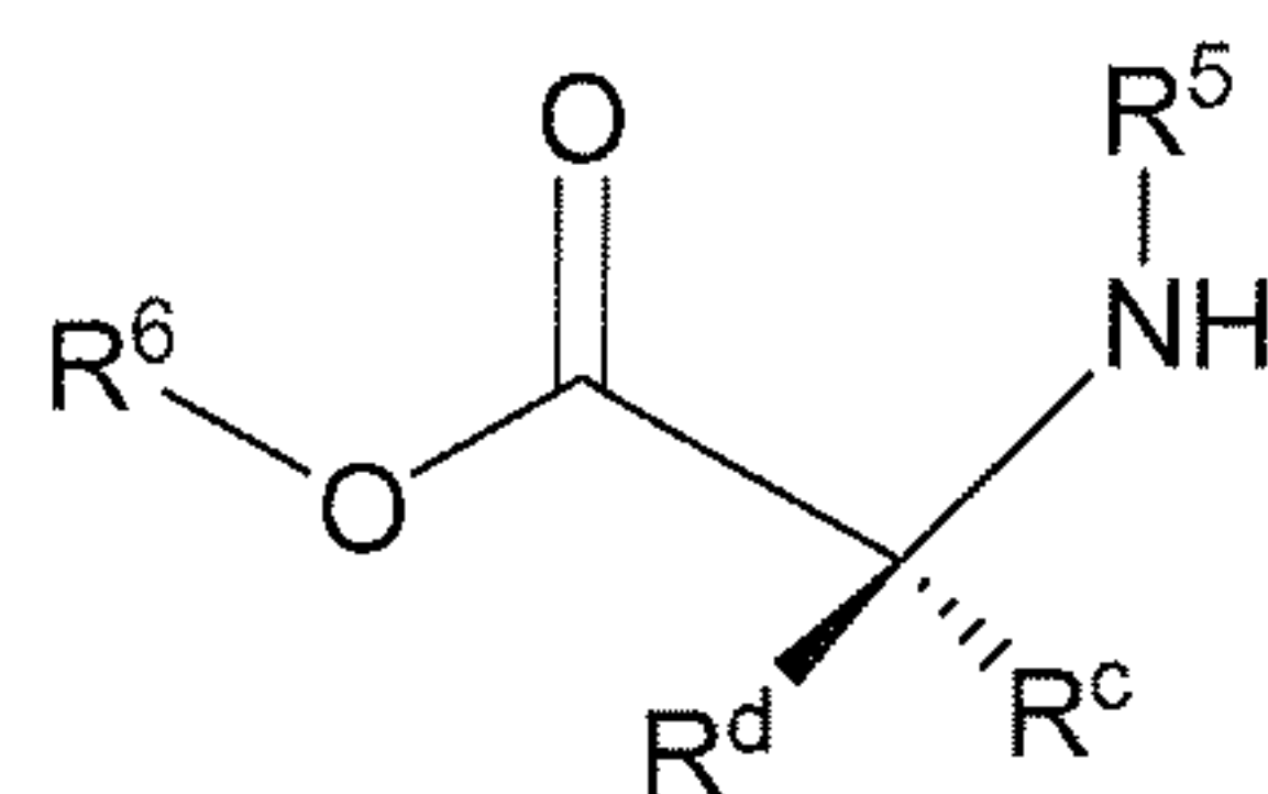
Formula IX
