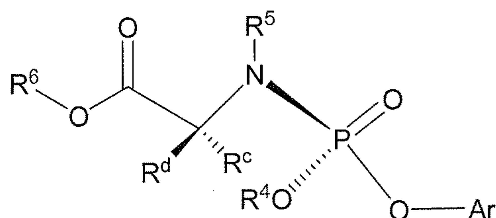
Formula IIIa
