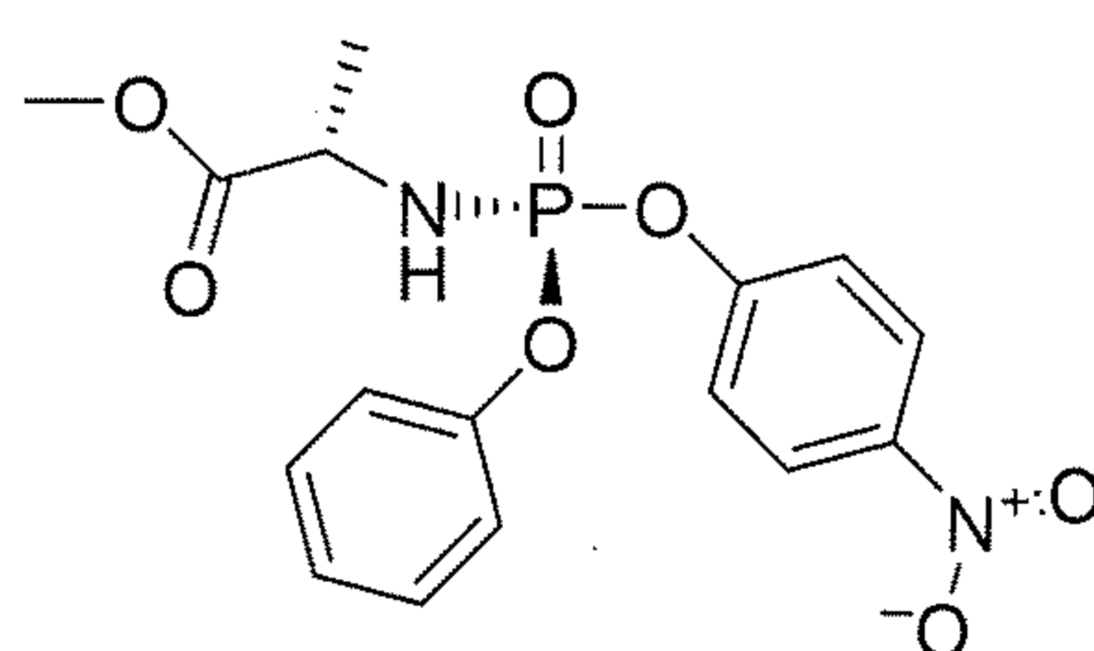
Compound 11
