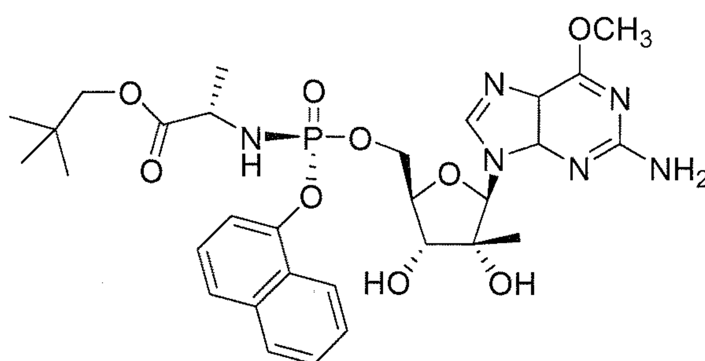
Compound 36
