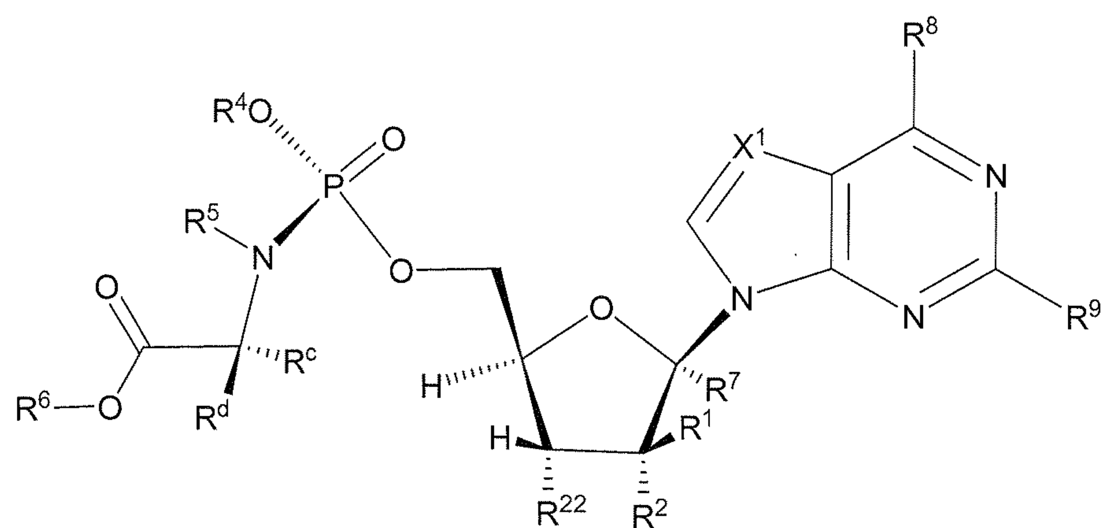
Formula XIb
