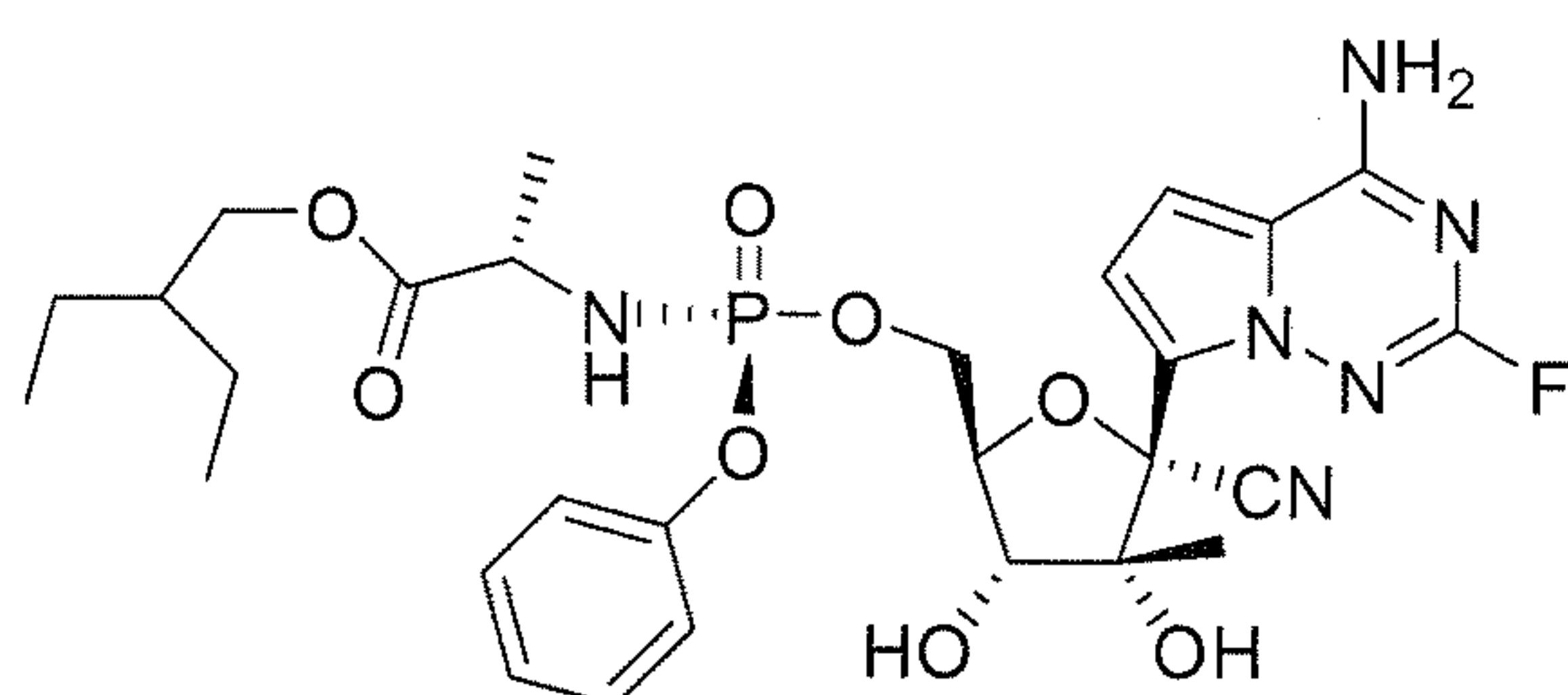
Compound 32
