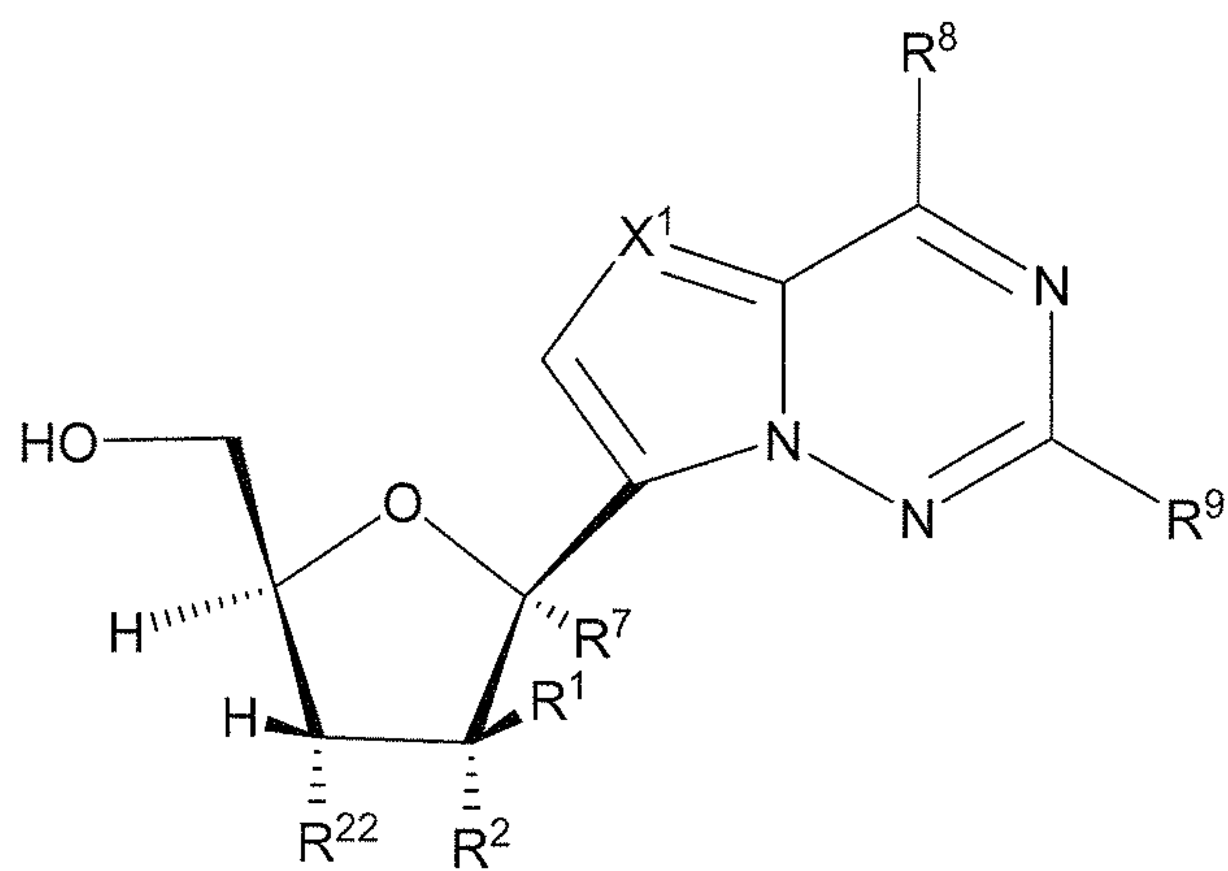
Formula VII
