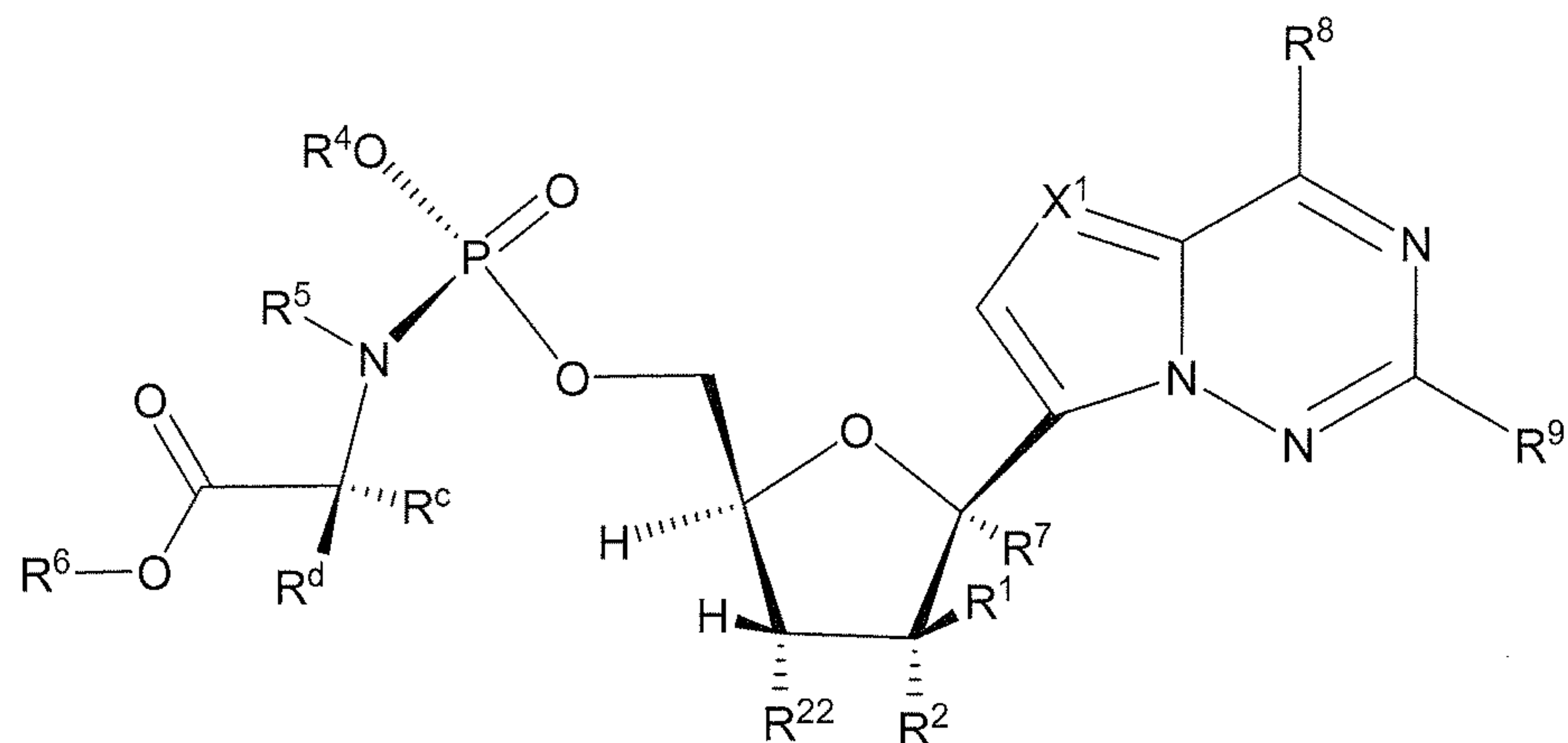
Formula VIb
