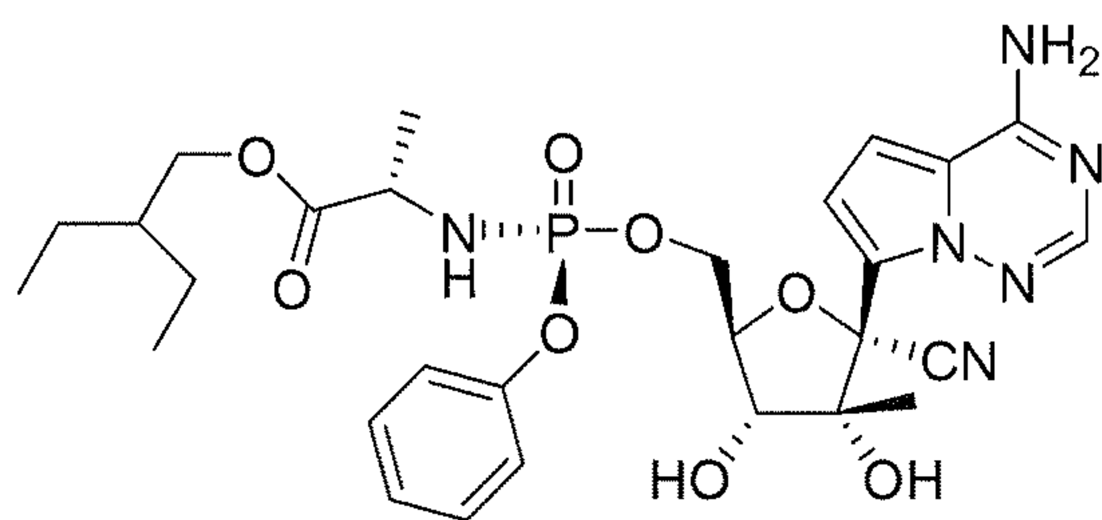
Compound 26
