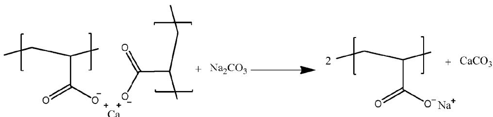
[045] Scheme 2. SAP recovery reaction using sodium or potassium carbonate
