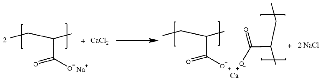
[043] Scheme 1. SAP reinforcement using calcium chloride
