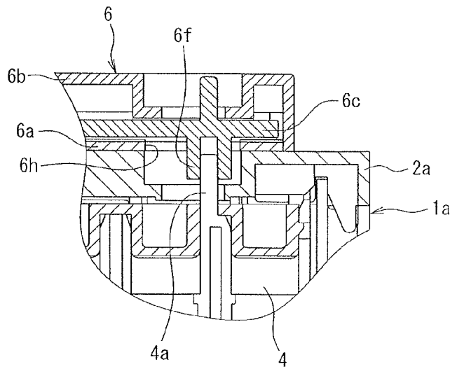
Fig. 13 Prior Art
