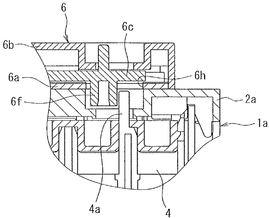
Fig. 14 Prior Art
