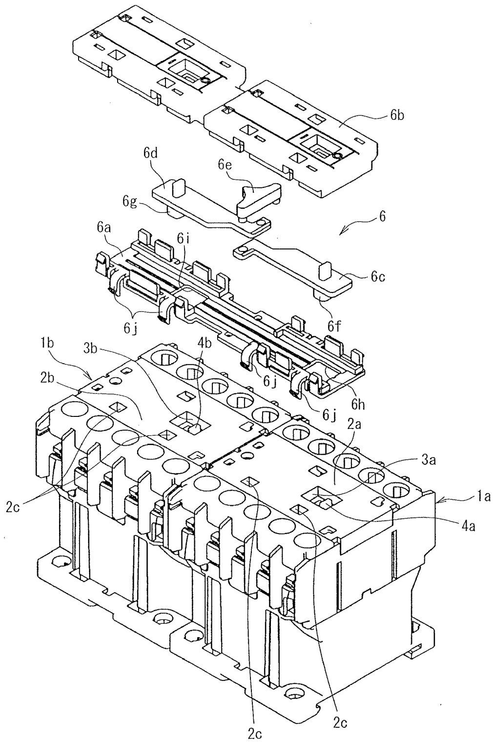
Fig. 11 Prior Art
