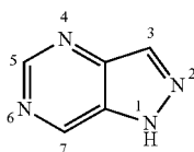
1H-pyrazolo[4,3-d]pyrimidine
