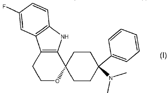
(1 r ,4 r )-6'-fluoro- N,N -dimethyl-4-phenyl-4',9'-dihydro-3' H -spiro[cyclohexane-1,1'-pyrano[3,4- b ]indol]-4-amine
