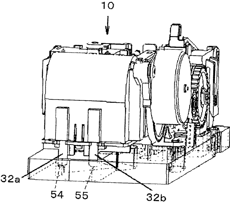
FIG. 19 (PRIOR ART)
