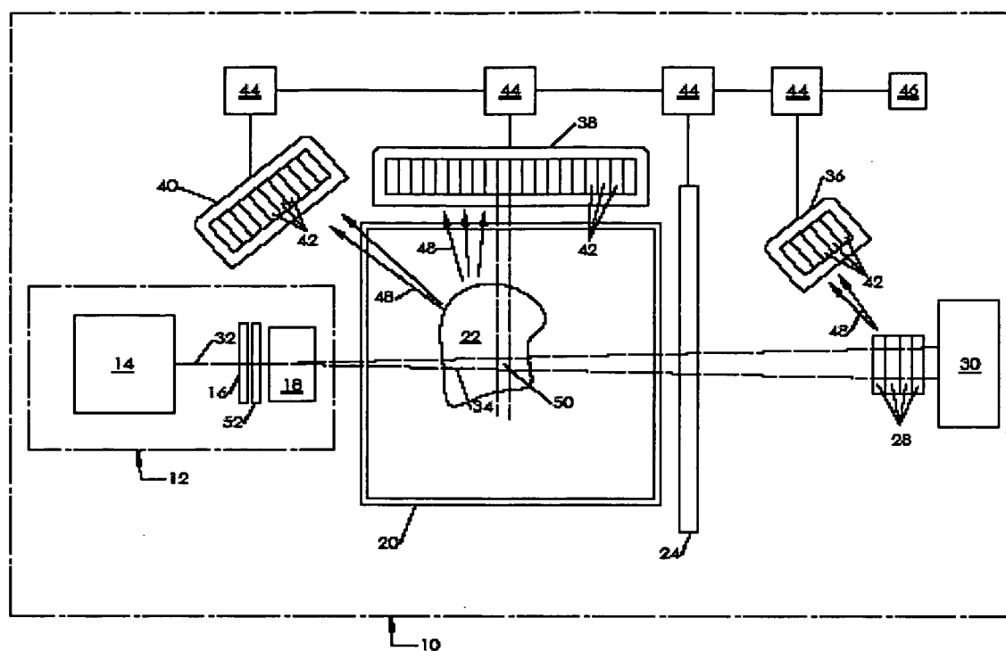
Figure 9. Schematic representation of Nuclear Resonance Fluorescence Scattering
