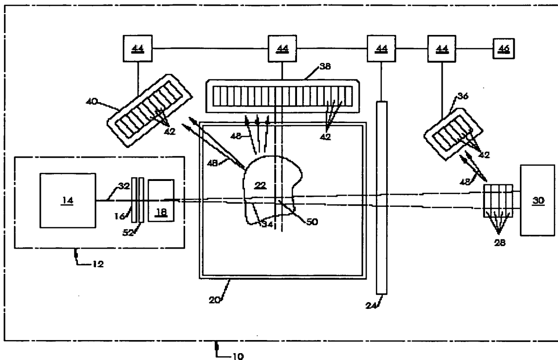
Schematic representation of Nuclear Resonance Fluorescence Scattering
