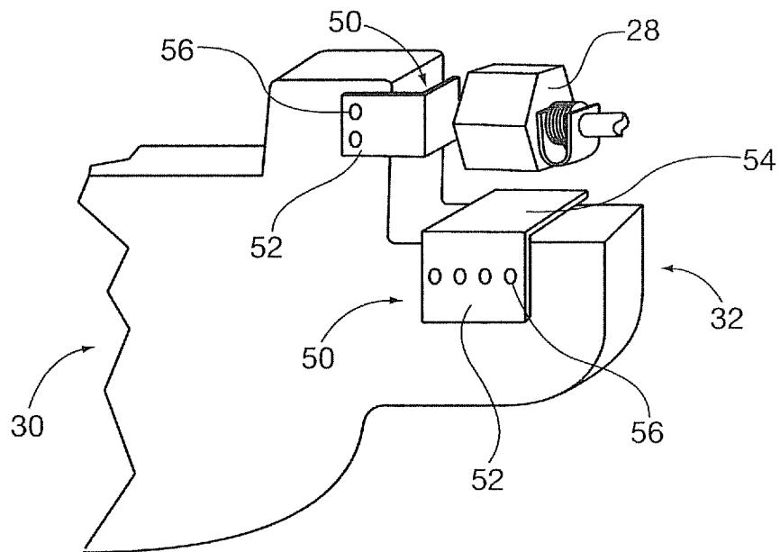
FIG. 3 PRIOR ART
