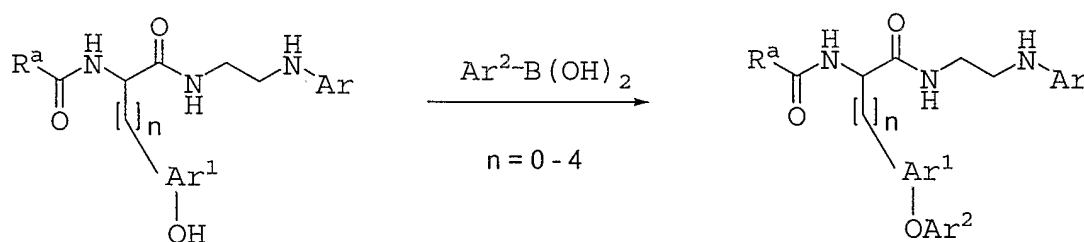
Scheme 6
