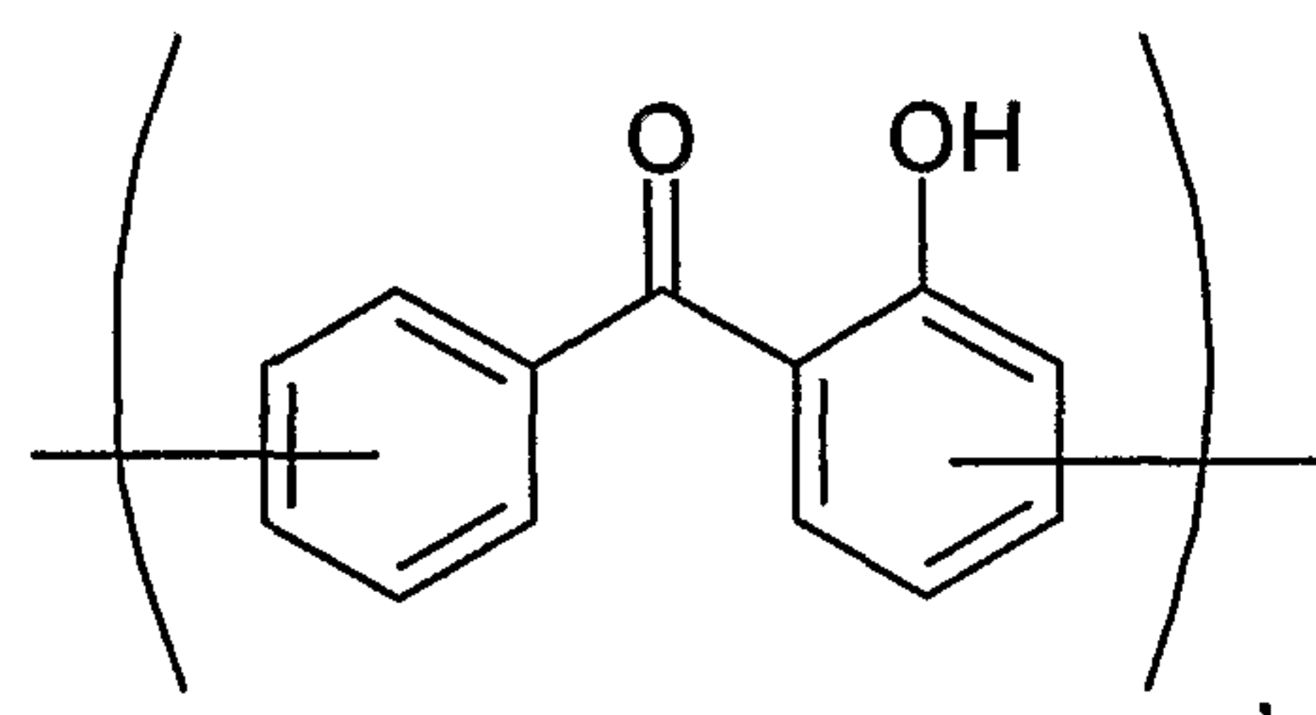
hydroxybenzophenone
