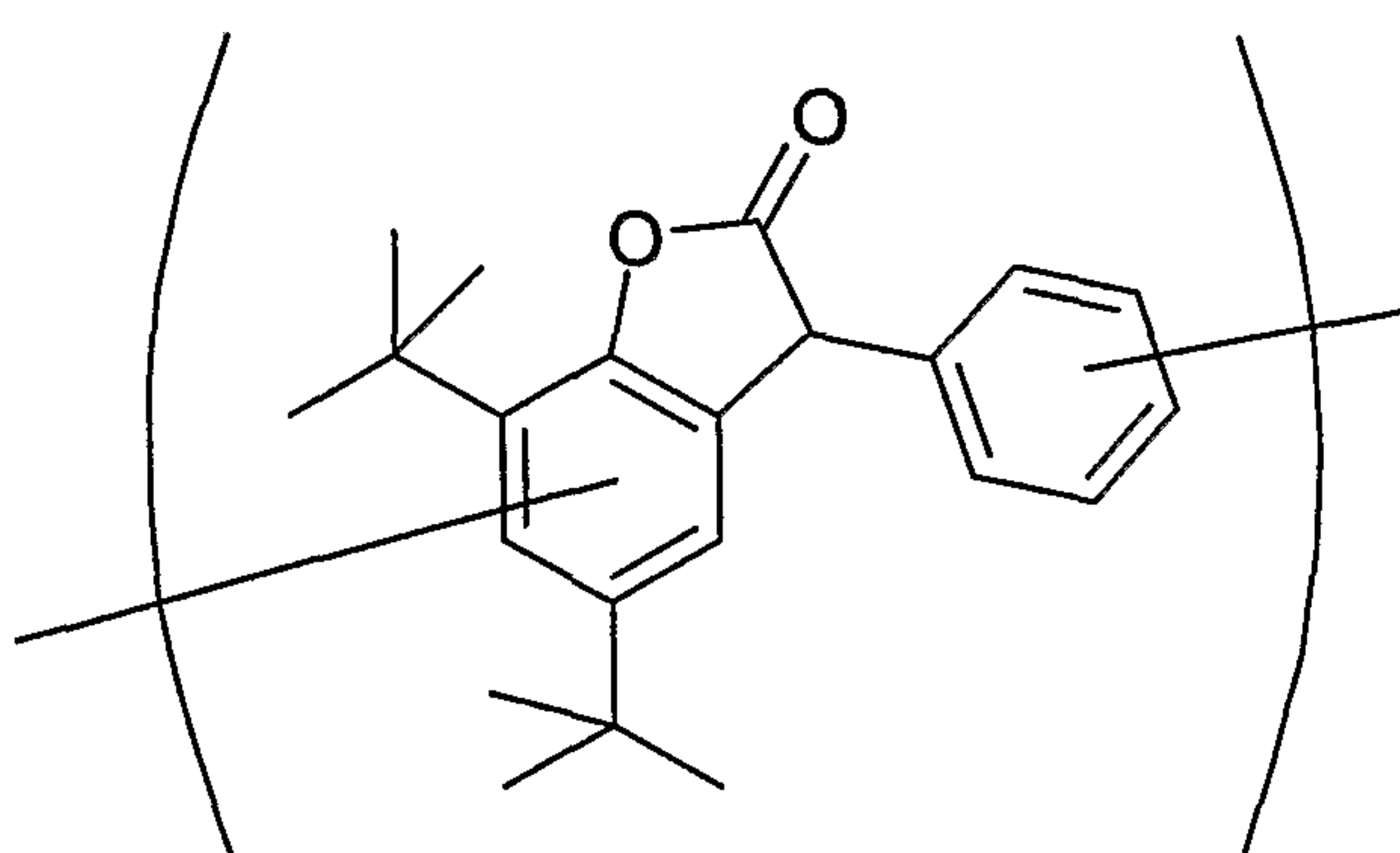
benzofuranone
