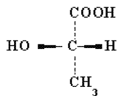
L(+) dextrorotatory lactic acid
