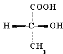
D(-) levorotatory lactic acid
