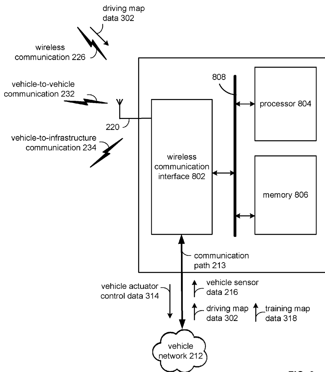
FIG. 8 Vehicle Control Unit 200
