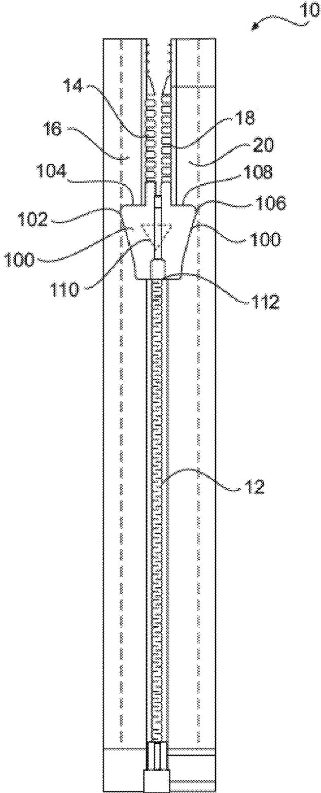
FIG. 2 (PRIOR ART)
