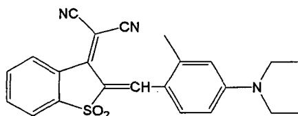
[Chemical formula 17]
