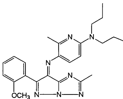
Azomethine compound M-I-I
