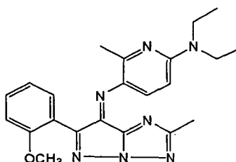
Azomethine compound M-I-VIII
