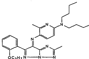
Azomethine compound M-I-VII
