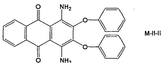
[Chemical formula 13]
