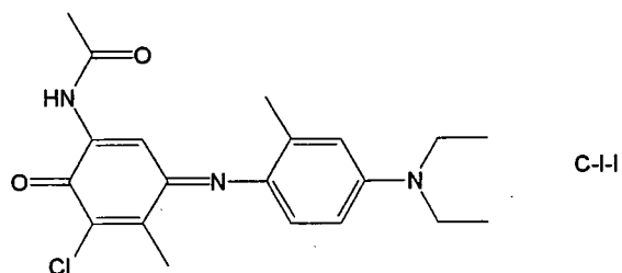
[Chemical formula 10]
