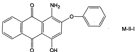
[Chemical formula 12]
