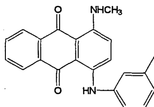
[Chemical formula 16]
