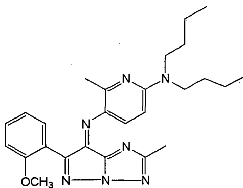
Azomethine compound M-I-II
