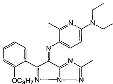
Azomethine compound M-I-V
