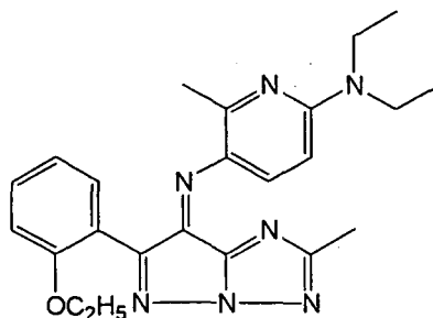
Azomethine compound M-I-III
