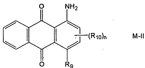
[Chemical formula 11]
