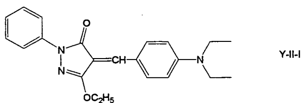
[Chemical formula 9]
