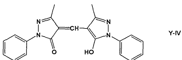
[Chemical formula 15]
