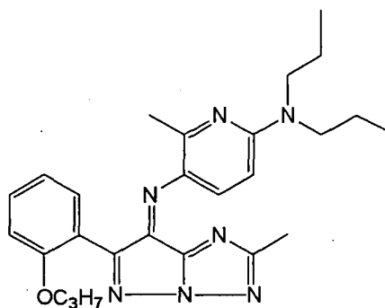
Azomethine compound M-I-VI
