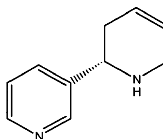
S-(-)-anatabine
