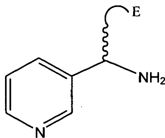
Formula IIIa
