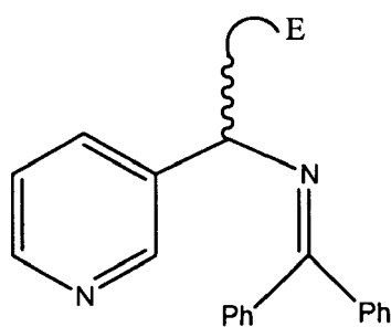
Formula IIa
