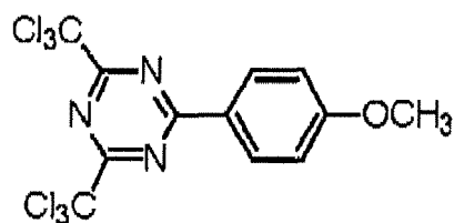
Polymerization Initiator (1)
