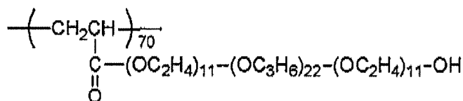
Fluorine-based surfactant (1)
