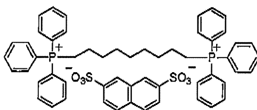
Phosphonium compound (1)
