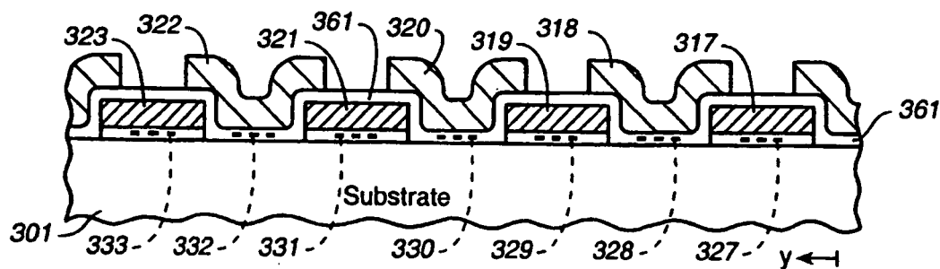
(SECTION X-X) FIG. 29B
