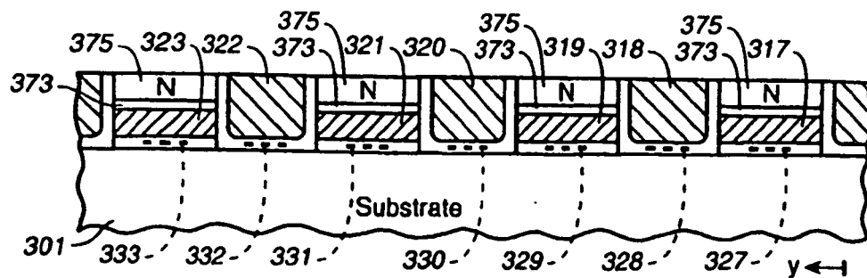
(SECTION X-X) FIG._30B
