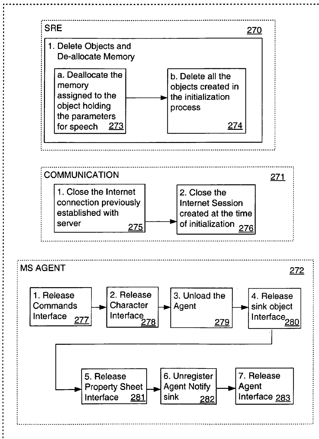
Fig. 4 Client-side Un-Initialization
