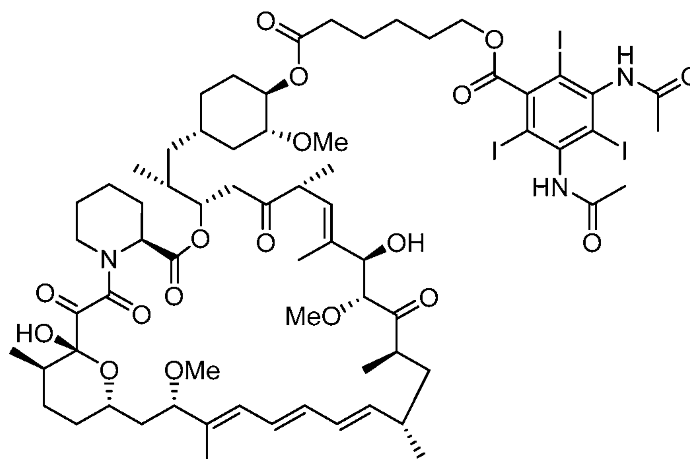
Formula 2.
