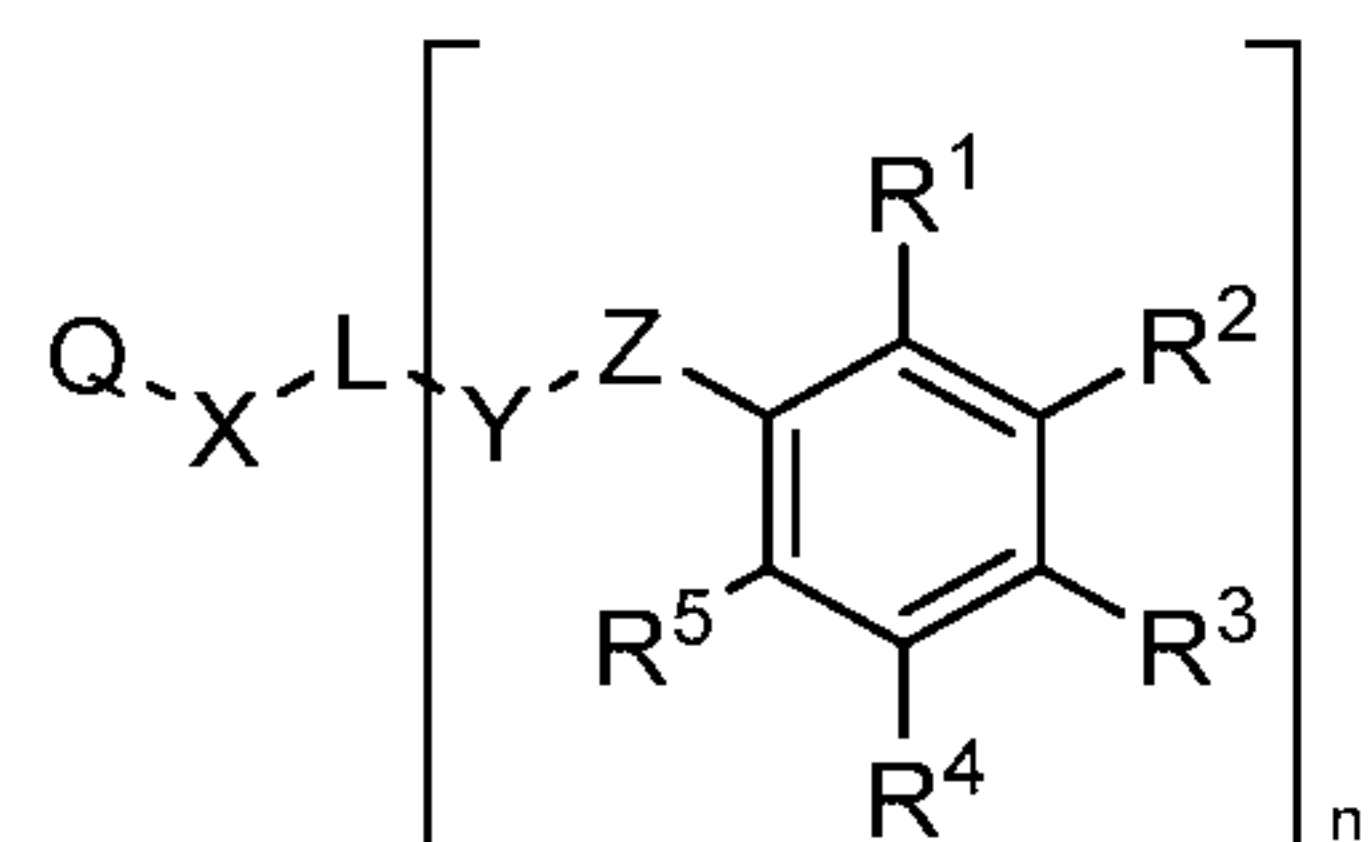
Formula 1
