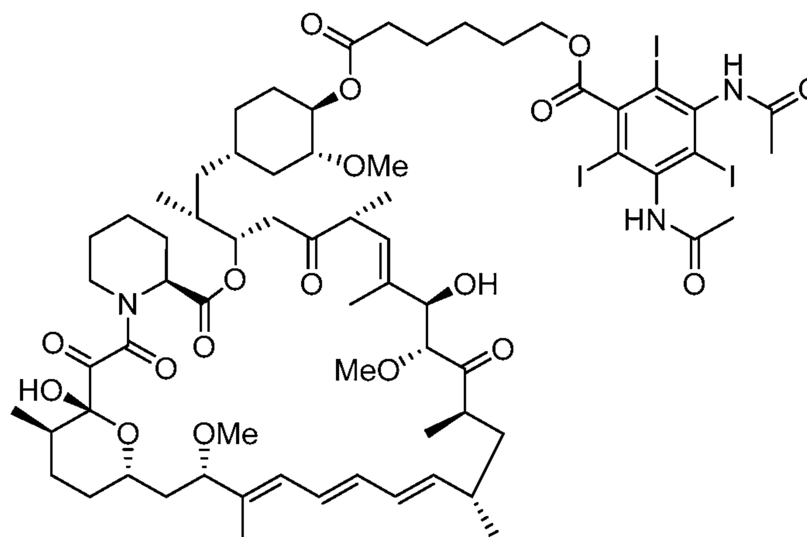
Formula 2.
