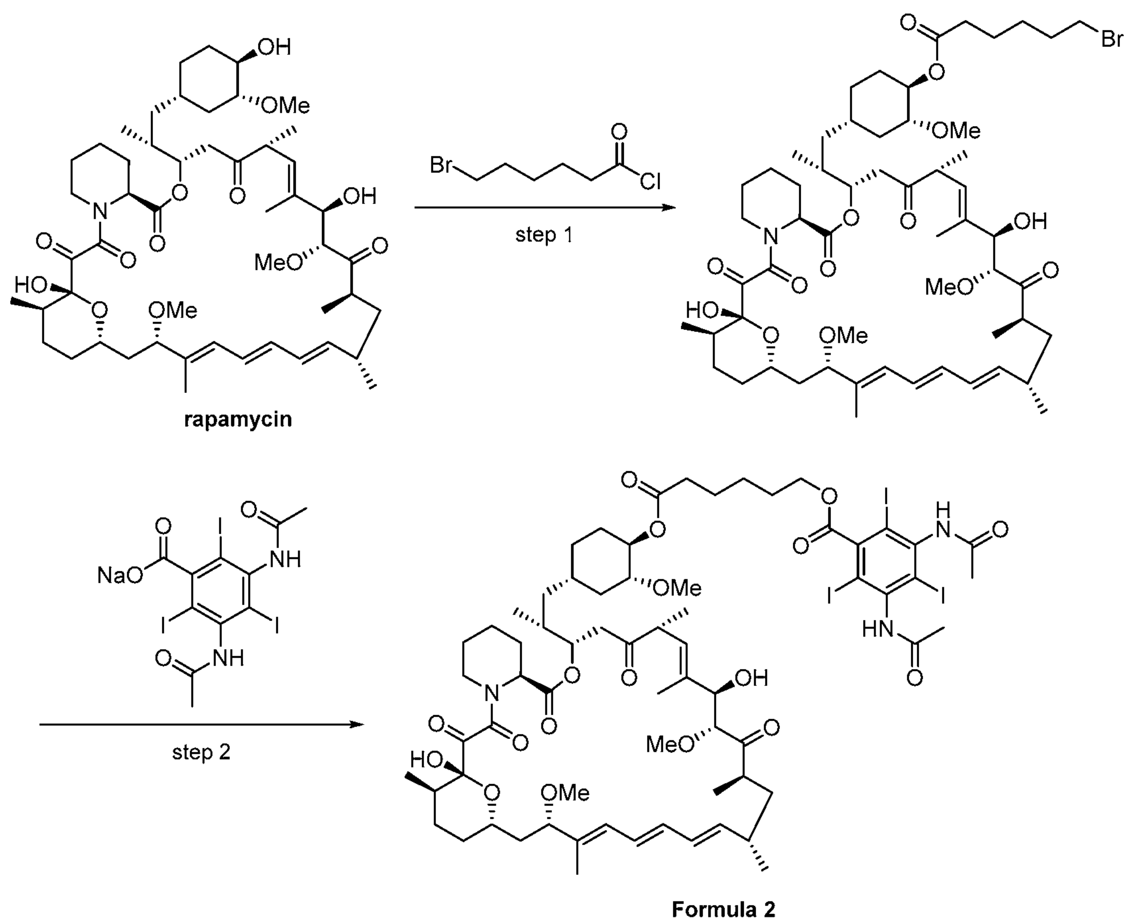
Scheme 1
