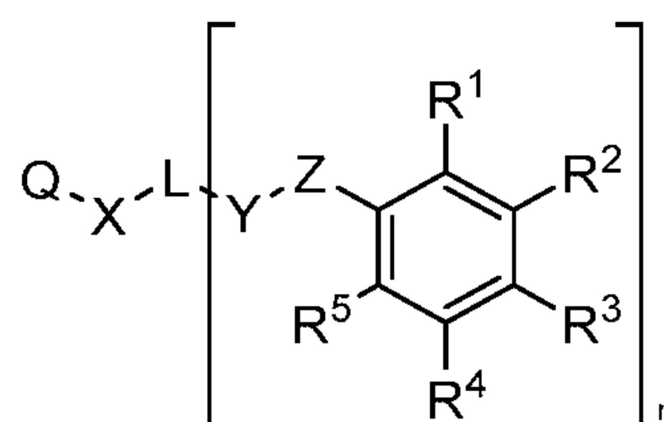
Formula 1
