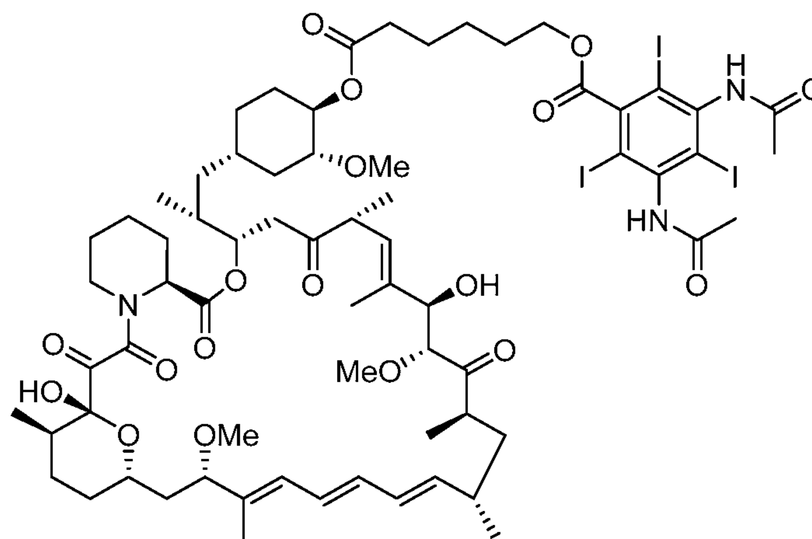
Formula 2.
