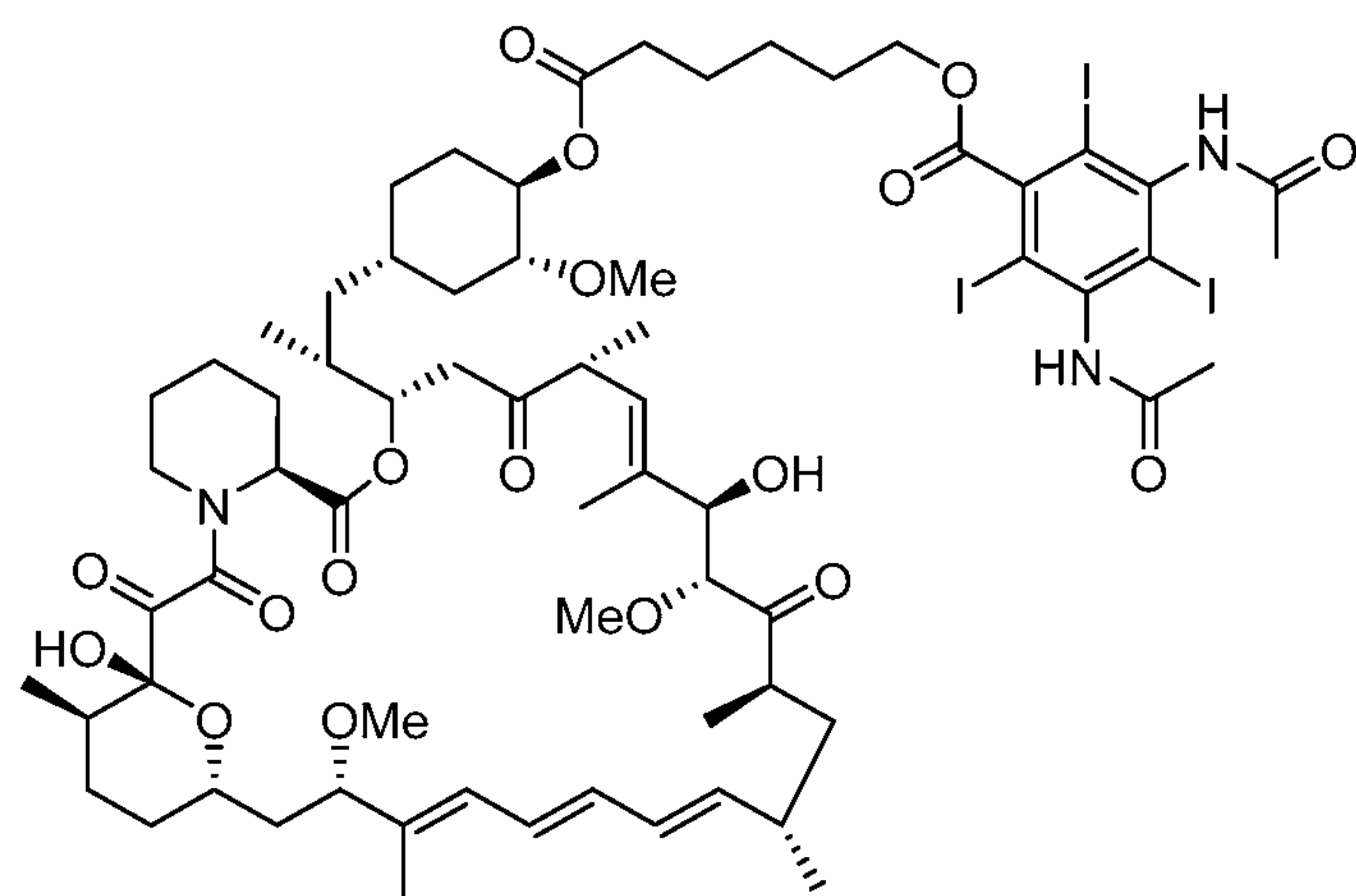
Formula 2.
