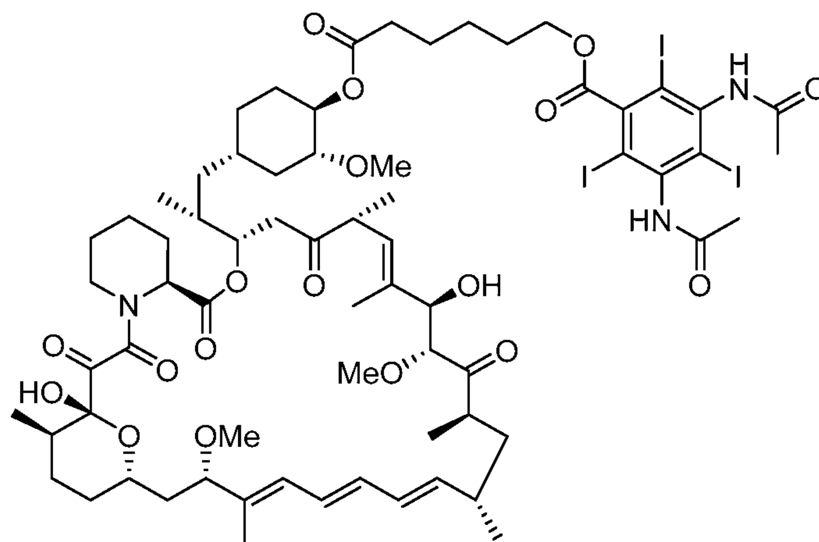
Formula 2.
