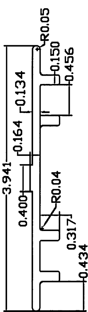
PART S1 26 - FIGURE 37
