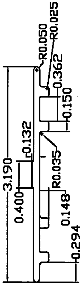
PART S 26 - FIGURE 38
