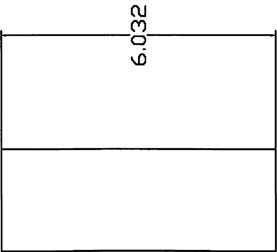
PART JA CUT LENGTH 6.032" 26 - FIGURE 41
