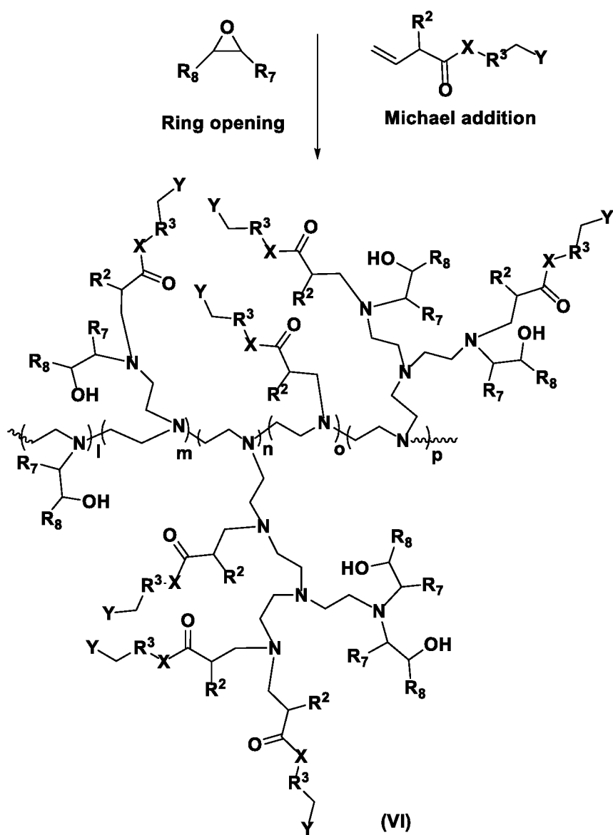
Branched Polyethyleimine
