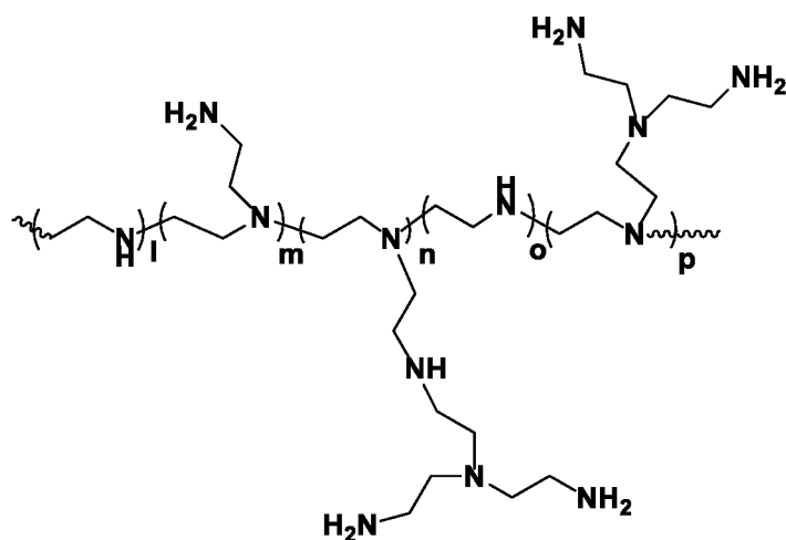
Branched Polyethyleimine
