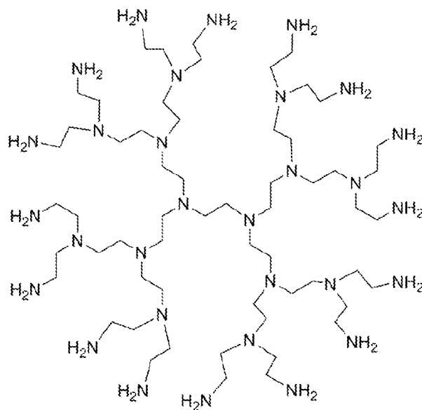
Fully Branched PEI
