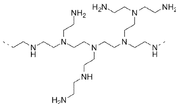
Exemplary Branched PEI
