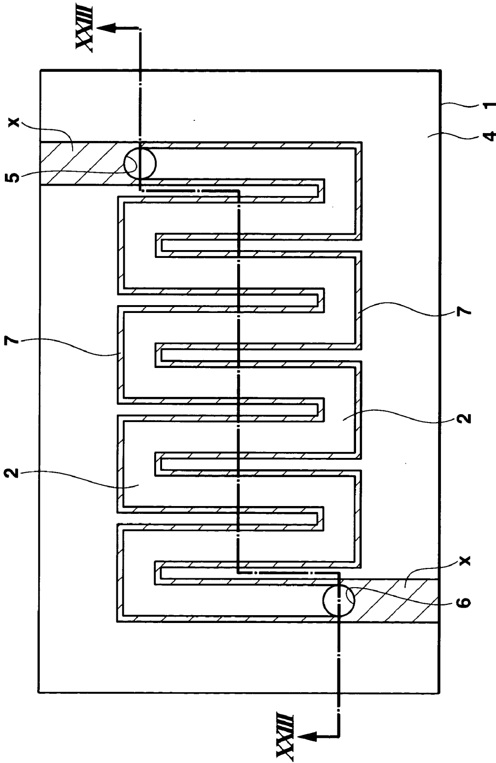
FIG.22 (RELATED ART)
