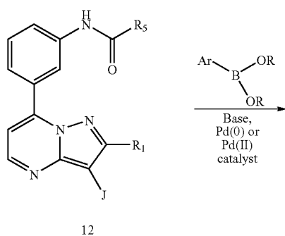
Scheme 4
