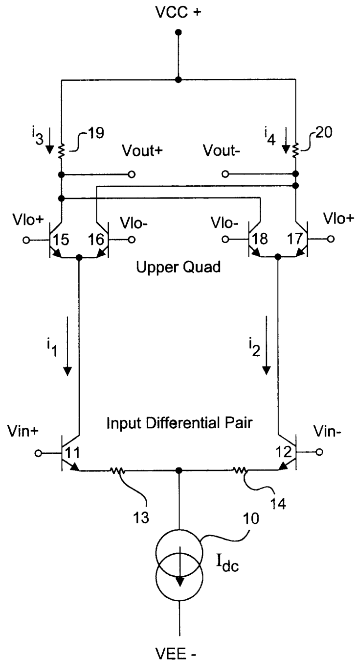
FIG. 1 PRIOR ART
