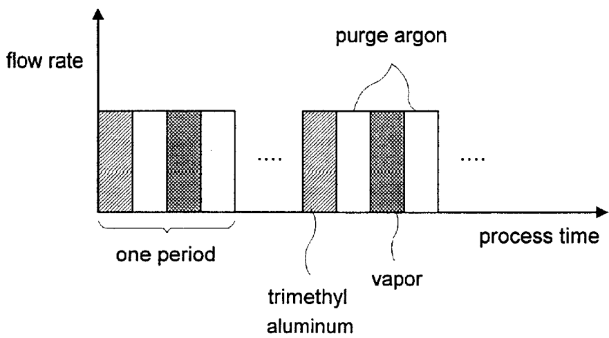
FIG. 2 (Prior Art)
