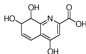
7,8-dihydro-7,8-dihydroxykynurenic acid
