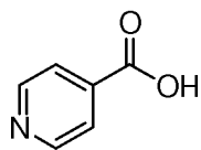
isonicotinic acid
