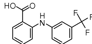
Flufenamic acid
