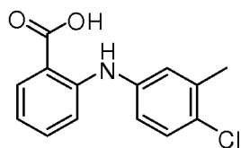
Tolfenamic acid
