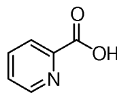
picolinic acid
