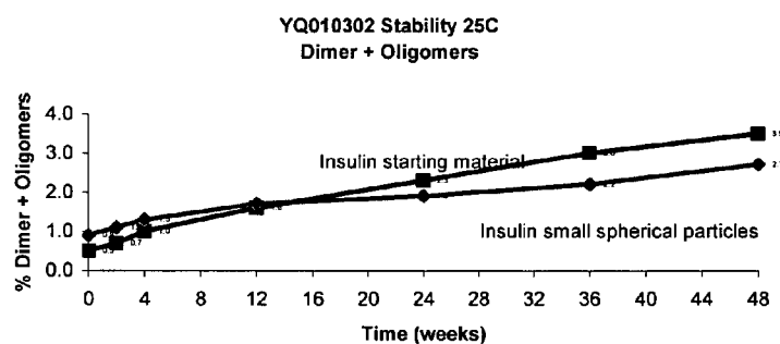
FIG. 32. At a storage temperature of 25°C, the percent insulin dimer and oligomer formation of the starting material is significantly greater compared to the insulin small spherical particles. This result indicates that the insulin small spherical particles are significantly more stable to chemical degradation than the starting material without the addition of stabilizing excipients.
