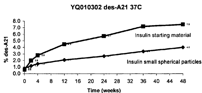
FIG. 31. At a storage temperature of 37°C, the percent A21-desamido insulin formation of the starting material is significantly greater compared to the insulin small spherical particles. This result indicates that the insulin small spherical particles are significantly more stable to chemical degradation than the starting material without the addition of stabilizing excipients.
