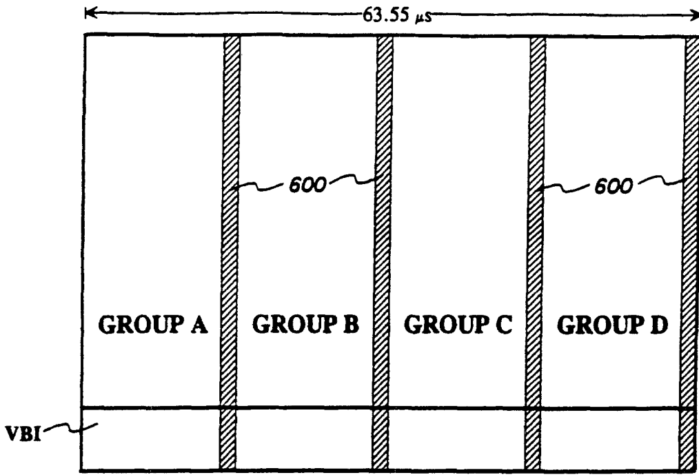
STAGGERED GROUPING IN TIME DOMAIN
