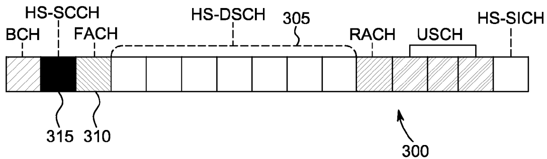
FIG. 3 PRIOR ART
