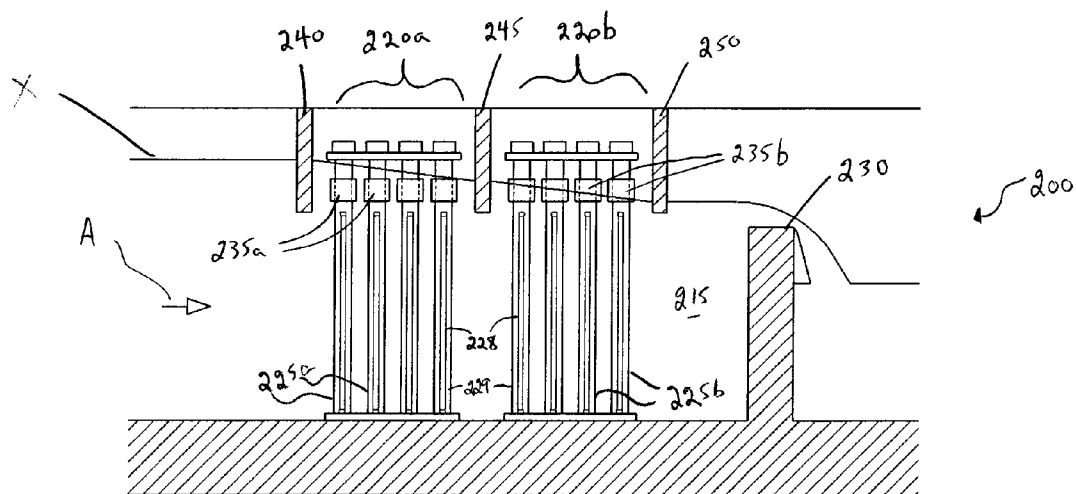
Baffled Surface with Wipers Figure 3
