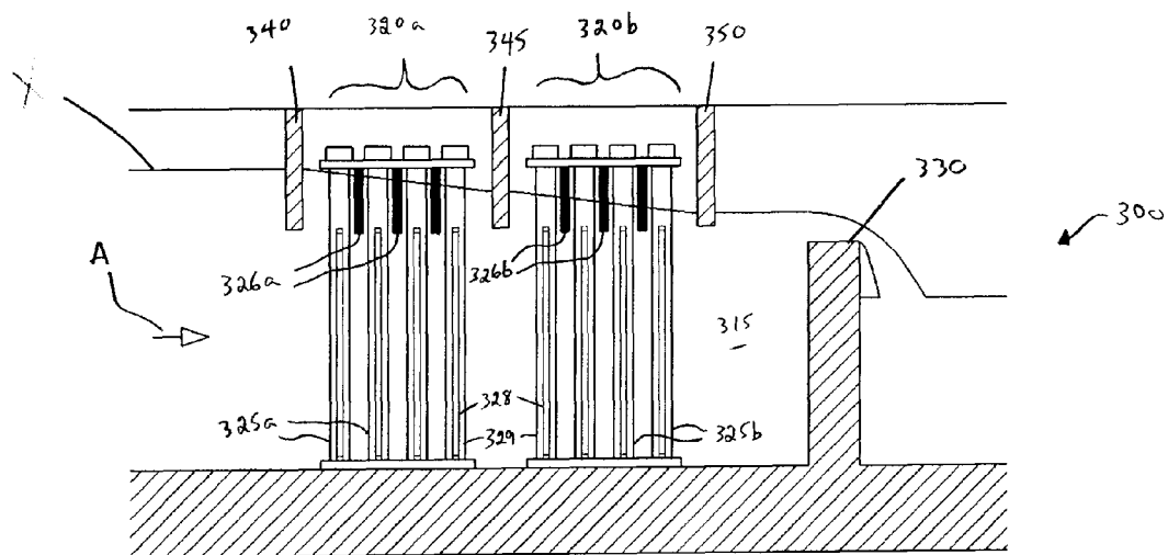
Baffled Surface with Ballasts Figure 4
