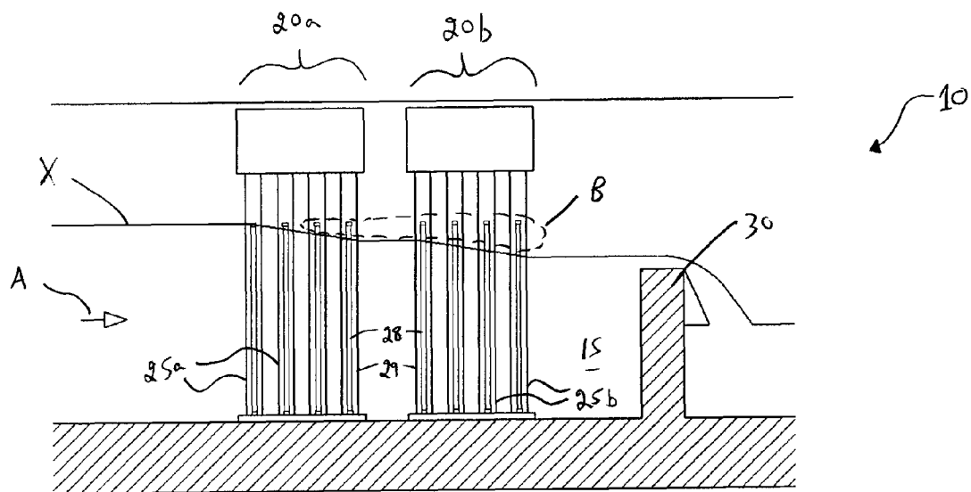
Free Surface – Common Enclosure Figure 1
