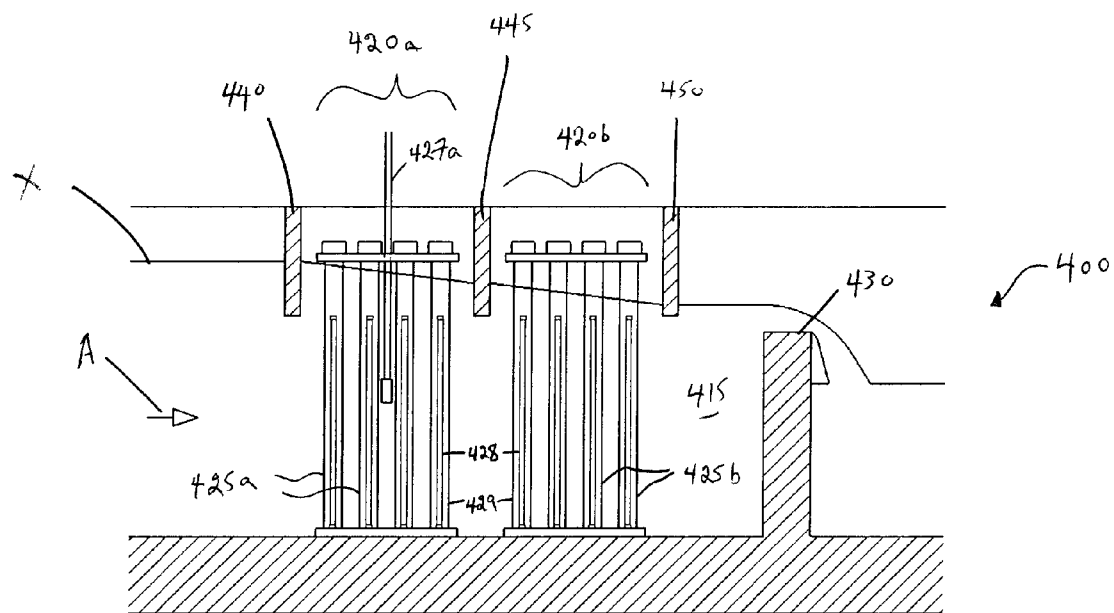
Baffled Surface with Dip Sensor Figure 5
