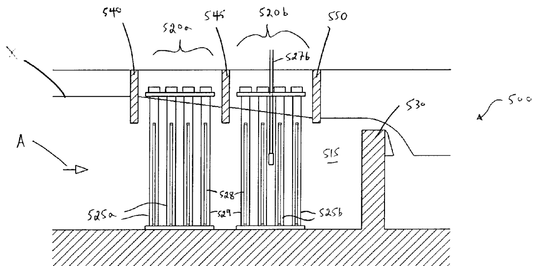
Baffled Surface with Dip Sensor relocated Figure 6
