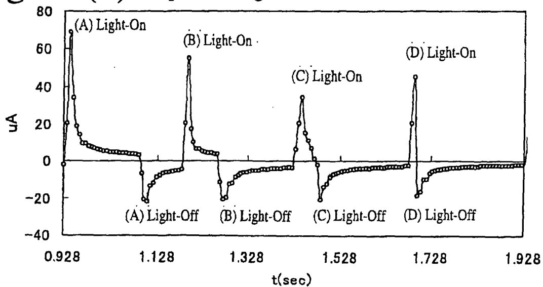
Fig. 18(b) Response to Light in one Turn
