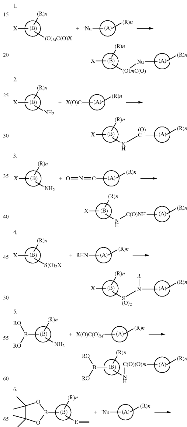
Scheme 4
