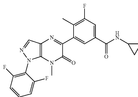
Synthesis of N-Cyclopropyl-3-(1-(2,6-difluorophenyl)-7-methyl-6-oxo-6,7-dihydro-1H-pyrazolo[4,3-b]pyrazin-5-yl)-5-fluoro-4-methylbenzamide
