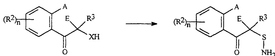
IVc (X is S)
