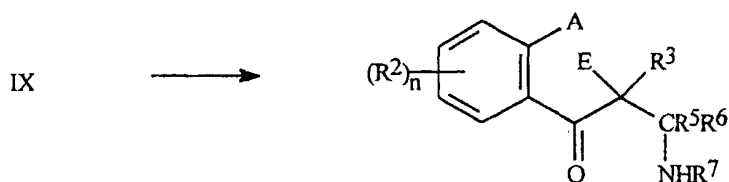
IVd (X is CR 5 R 6 )
