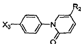
Subgenus III;
