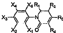
Genus Ia;
