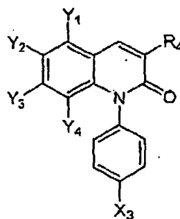
Genus VII
