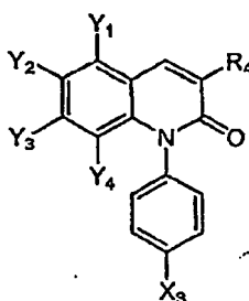
Genus VII
