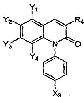
Genus VII
