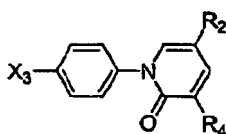
Genus Ic;
