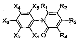
Genus Ia;
