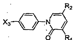
Genus Ic;
