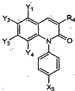
Genus VII
