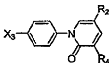
Genus Ib;
