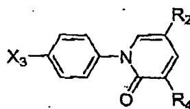
Genus Ic;
