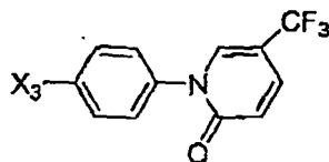
Subgenus V
