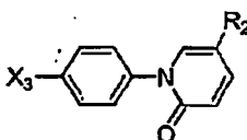
Subgenus III;
