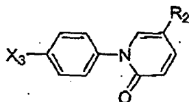
Subgenus III;
