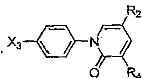
Genus Ib;
