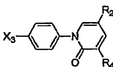
Subgenus II;
