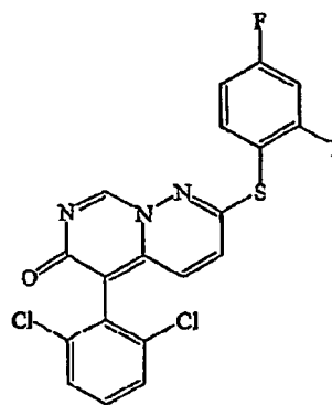
P8 VX-745
