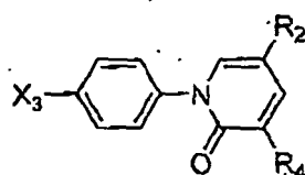
Subgenus II;
