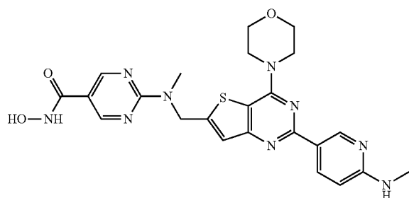
Compound 3
