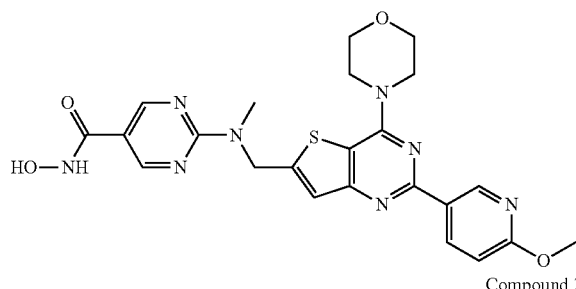
Compound 2
