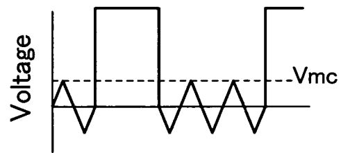
Triangle Wave
