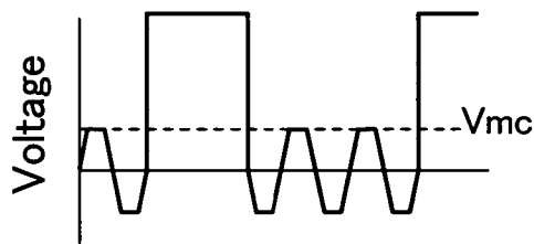
Sine Wave 2 (Limited Peak Voltage)
