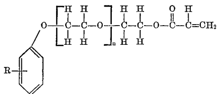
ALKYLPHENOXYETHYLENEOXYETHYL ACRYLATE
