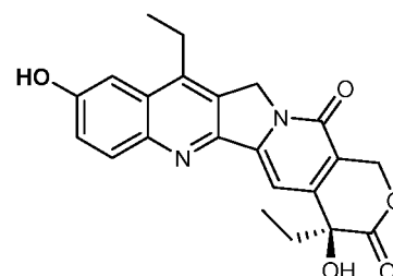
SN38 Topoisomerase 1 inhibitor
