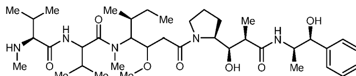
Monomethyl Auristatin E Peptide based antimitotic agent
