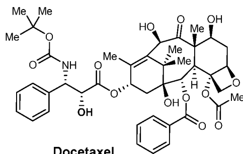
Docetaxel Microtubule inhibitor
