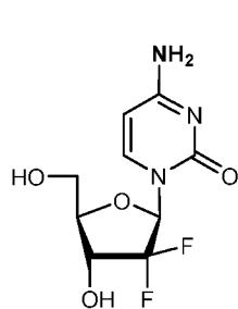
Gemcitabine Nucleoside analog
