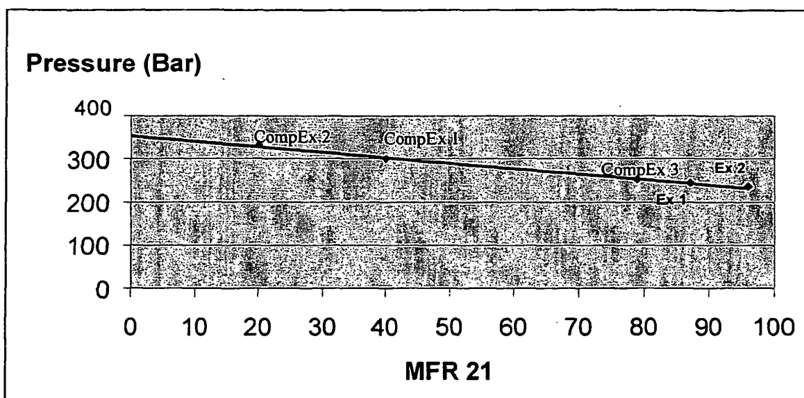
Fig. 1: Extruder pressure as a function of MFR 21
