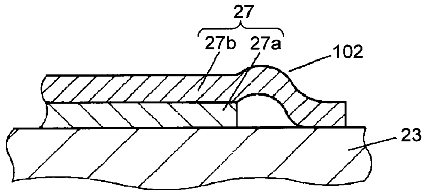
FIG. 6 PRIOR ART
