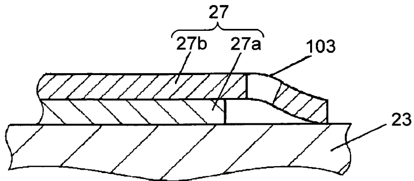
FIG. 7 PRIOR ART
