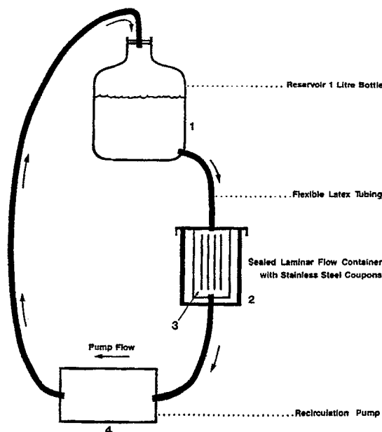
Diagram of Continuous Flow Pump System
