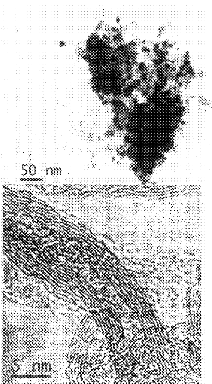
Figure 4: (A) Typical transmission electron micrograph (TEM) of a direct current PECVD produced nanotube and (B) High magnification of nanolube showing aligned graphene walls along nanotube axis, produced according to an embodiment of the present invention.
