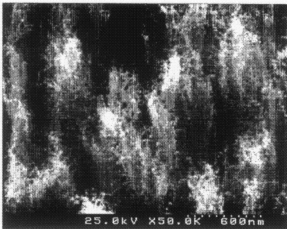
Figure 3: Typical scanning electron micrograph (SEM) of Carbon nanotubes produced at below 350°C temperature in direct current acetylene/nitrogen/hydrogen plasma on Ni catalyst particles, according to an embodiment of the present invention.
