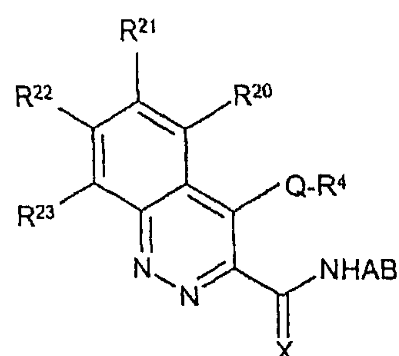
(Ic)
