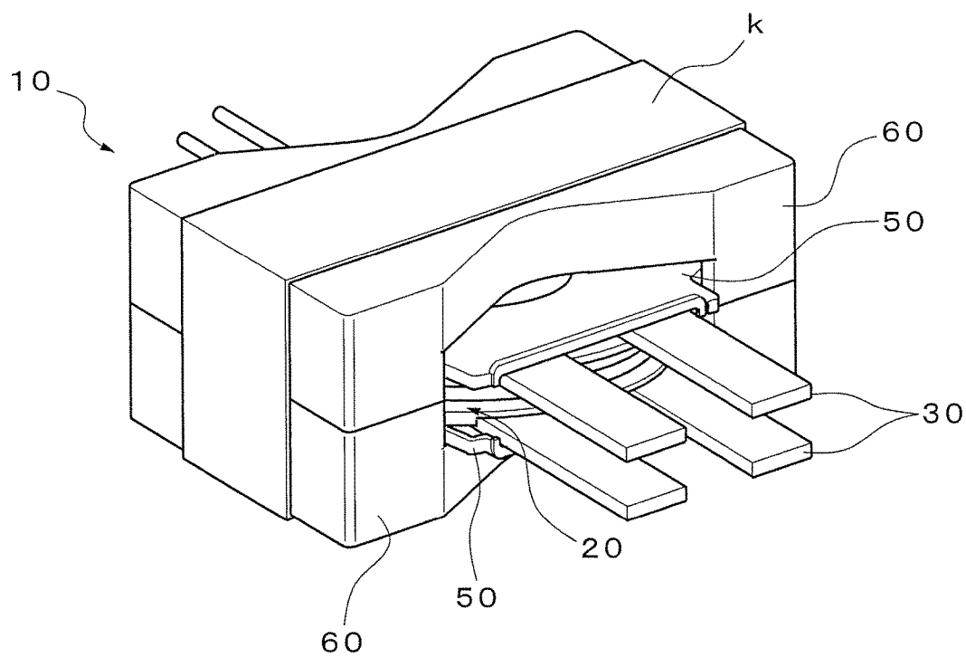
FIG. 7 (PRIOR ART)
