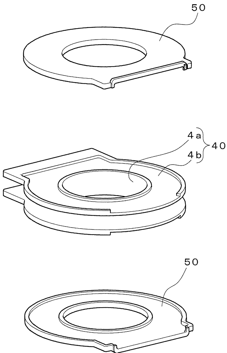
FIG. 6 (PRIOR ART)
