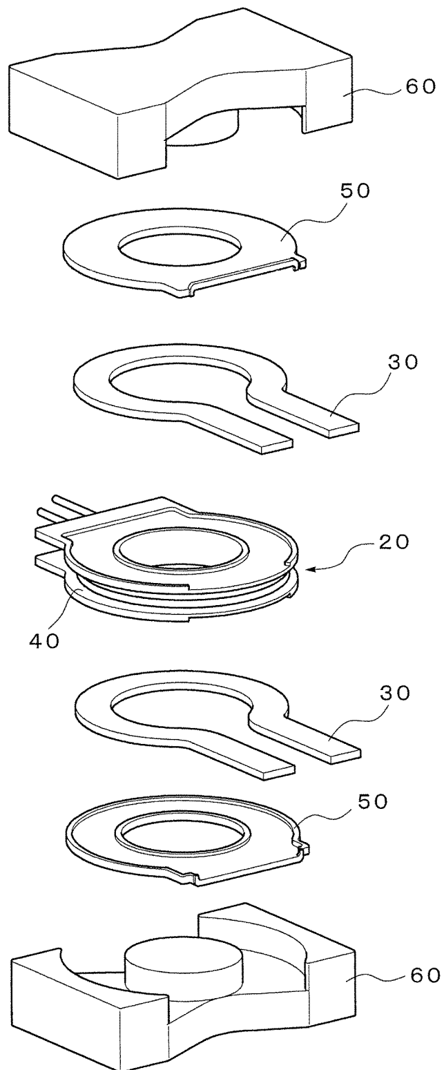
FIG. 8 (PRIOR ART)
