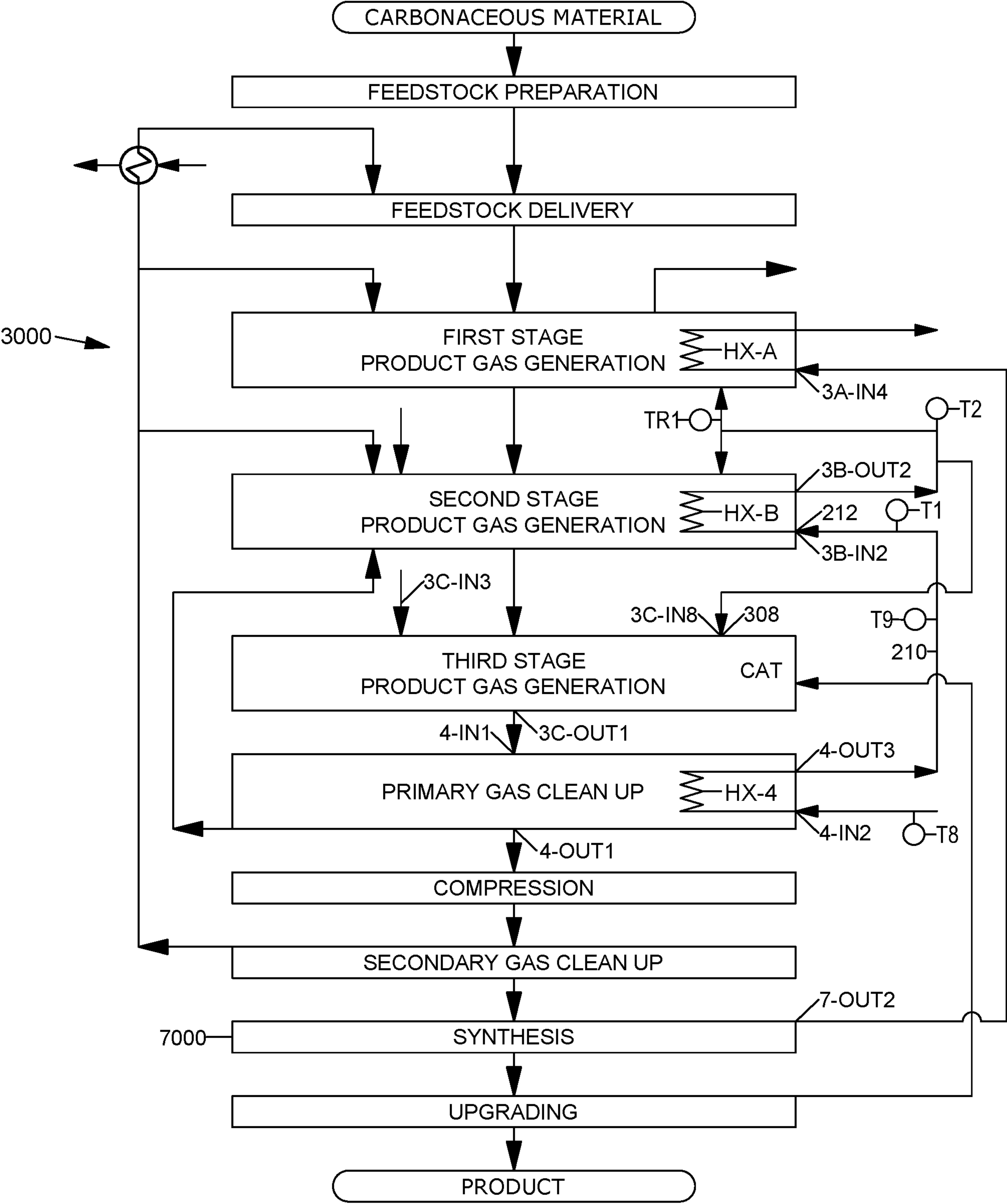
FIGURE 26 REFINERY SUPERSTRUCTURE (RSS)
