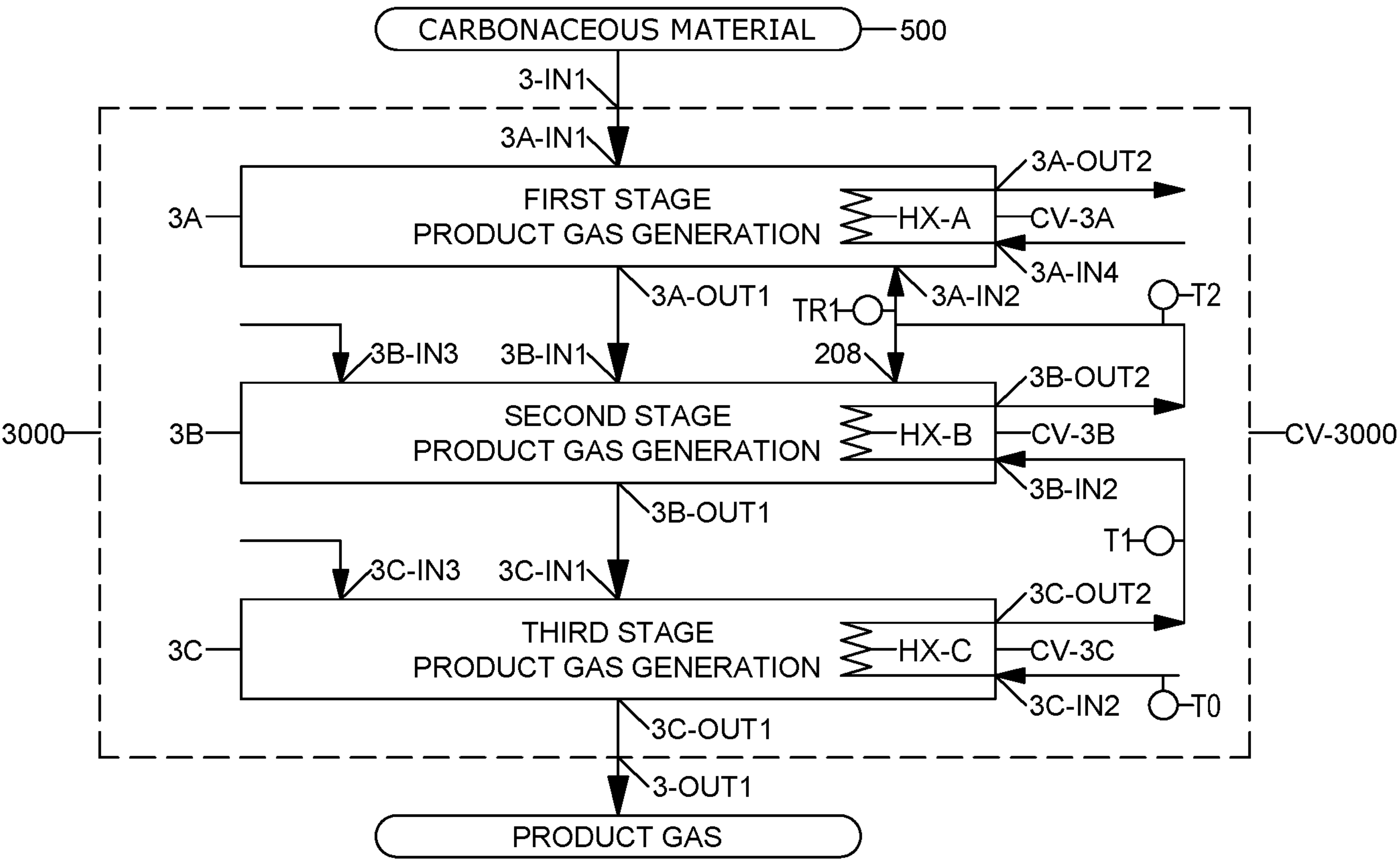
FIGURE 1 PRODUCT GAS GENERATION SUBSYSTEMS 3A & 3B & 3C
