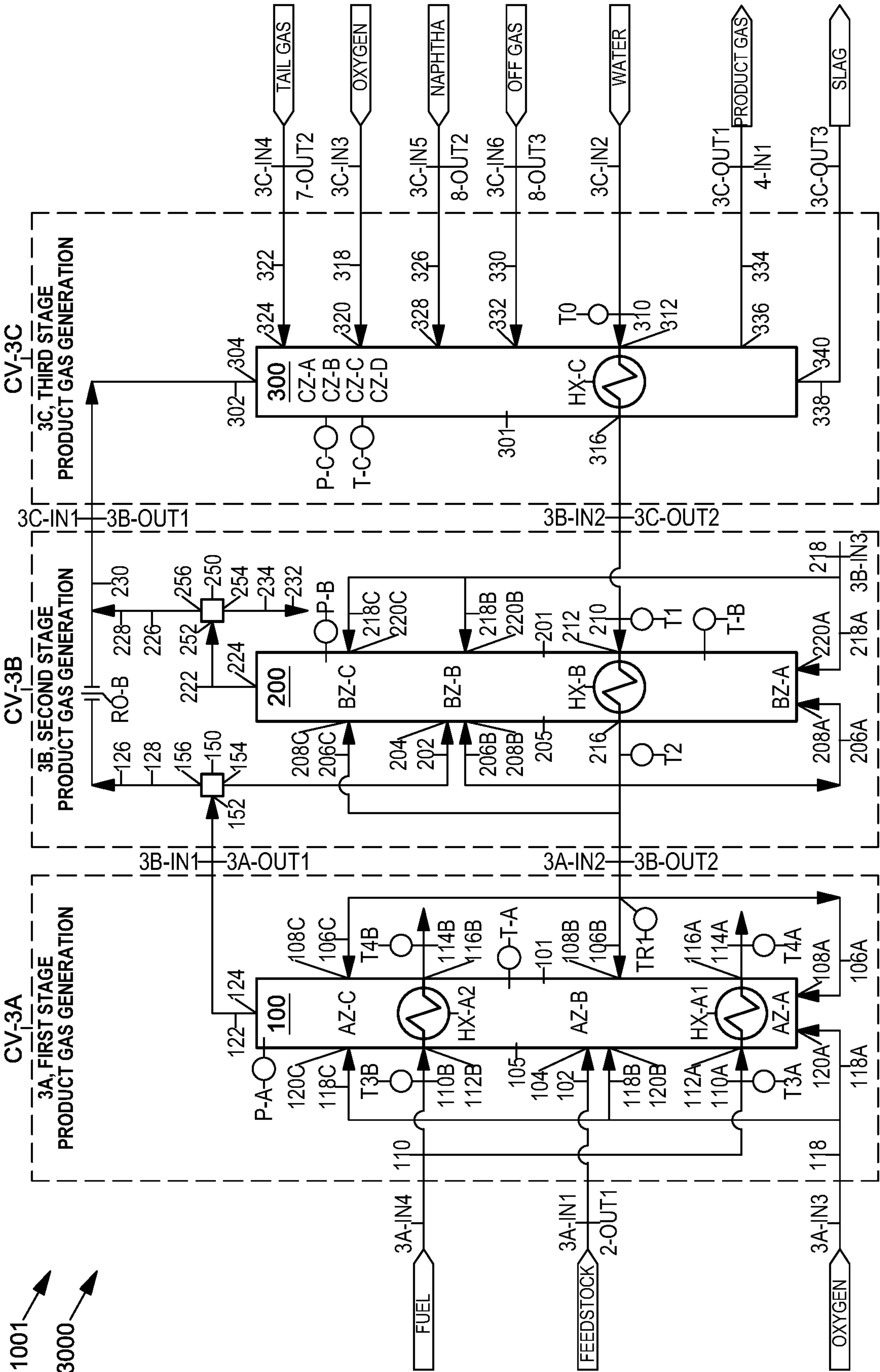
FIGURE 3 PRODUCT GAS GENERATION (3A & 3B & 3C)
