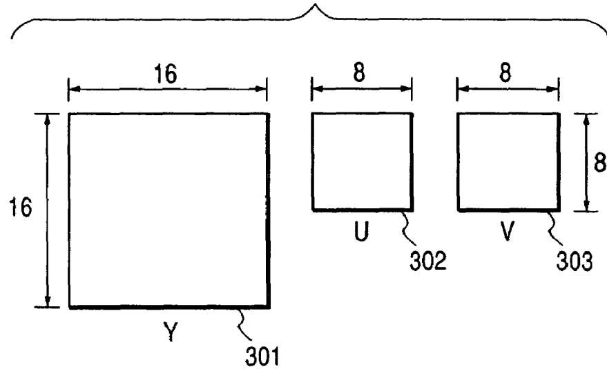
FIG. 3 (PRIOR ART)
