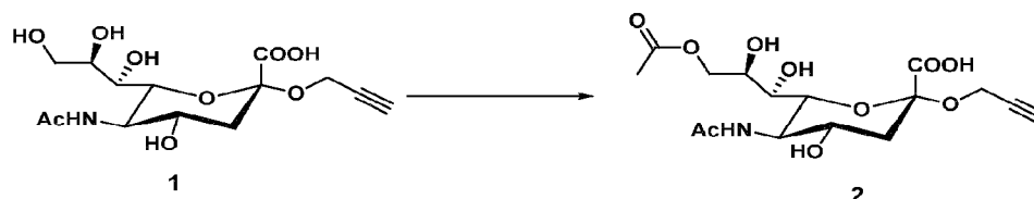
Scheme 2: Synthesis of intermediate compound 002
