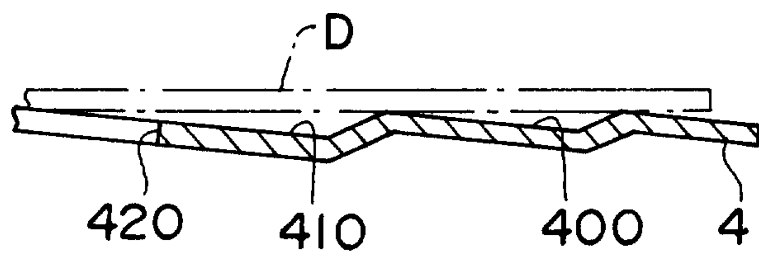
FIG.45 PRIOR ART
