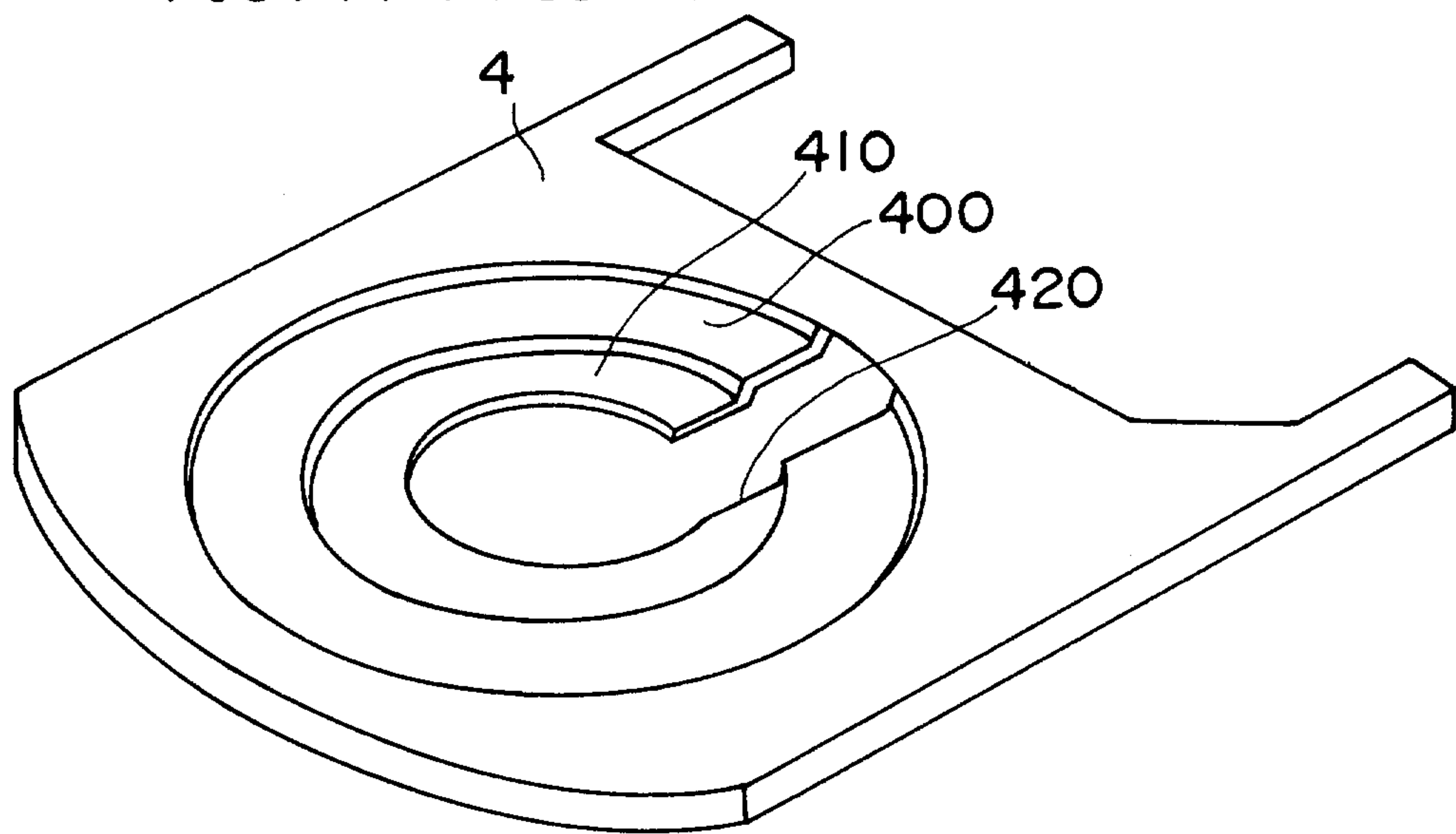
FIG.44 PRIOR ART
