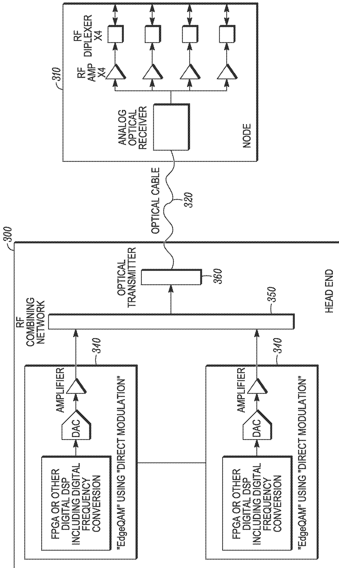
EdgeQAM BASED VIDEO TRANSMISSION SYSTEM
